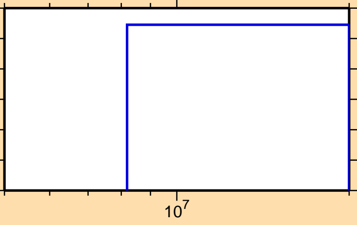
\sigma vs. E for ^{156}\text{Sm}(n,2np)
