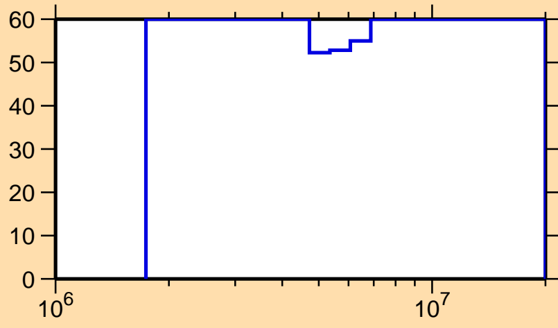
\Delta\sigma/\sigma vs. E for ^{157}\text{Sm}(n,\gamma)
