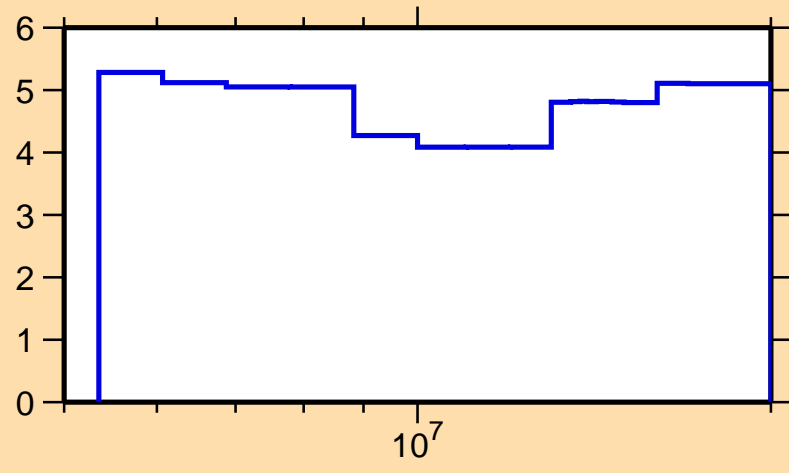
\Delta\sigma/\sigma vs. E for ^{157}\text{Sm}(n,\text{nonel.})
