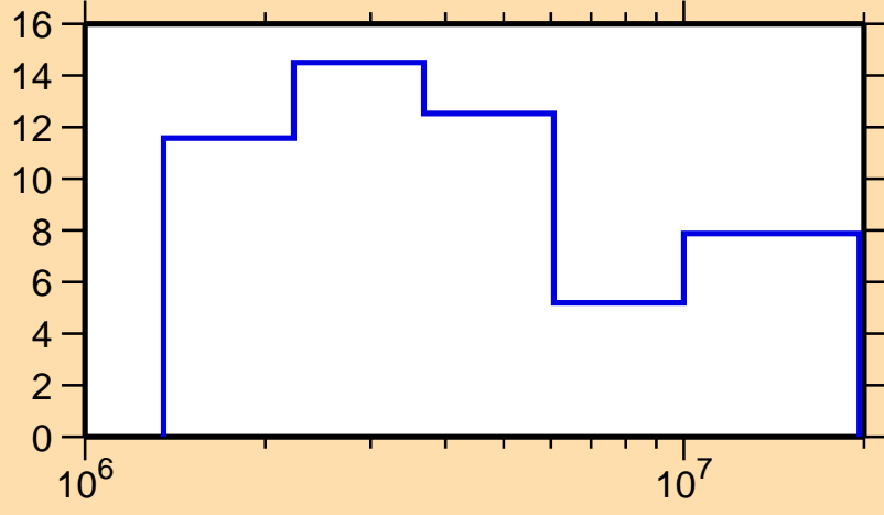
\Delta\sigma/\sigma vs. E for ^{157}\text{Sm}(n, el.)
