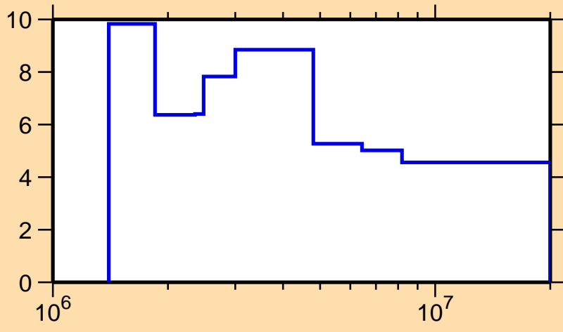
\Delta\sigma/\sigma vs. E for ^{157}\text{Sm}(n, n_{\text{onel}}) .
