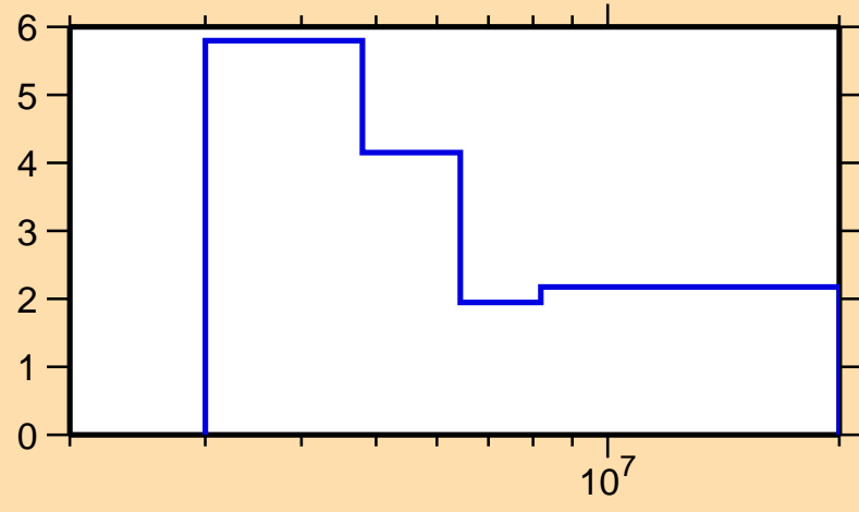
\Delta\sigma/\sigma vs. E for ^{157}\text{Sm}(n,\text{tot.})
