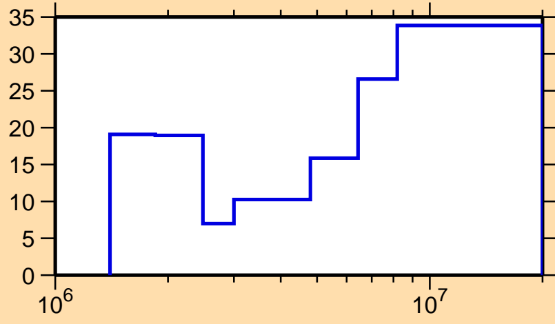
\Delta\sigma/\sigma vs. E for ^{157}\text{Sm}(n,ncont.)
