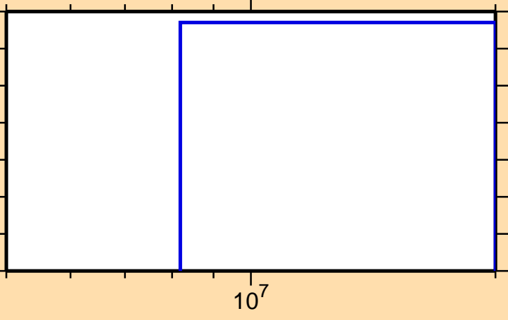
\sigma vs. E for ^{157}\text{Sm}(n,np)
