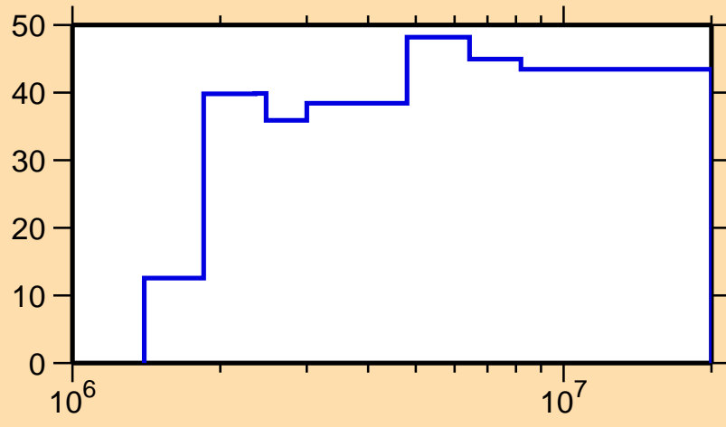
\Delta\sigma/\sigma vs. E for ^{157}\text{Sm}(n,n_1)
