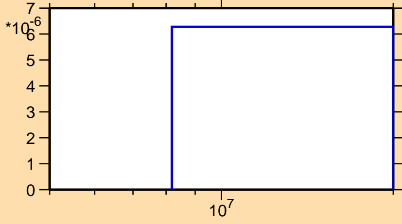
\sigma vs. E for ^{158}\text{Sm}(n,np)
