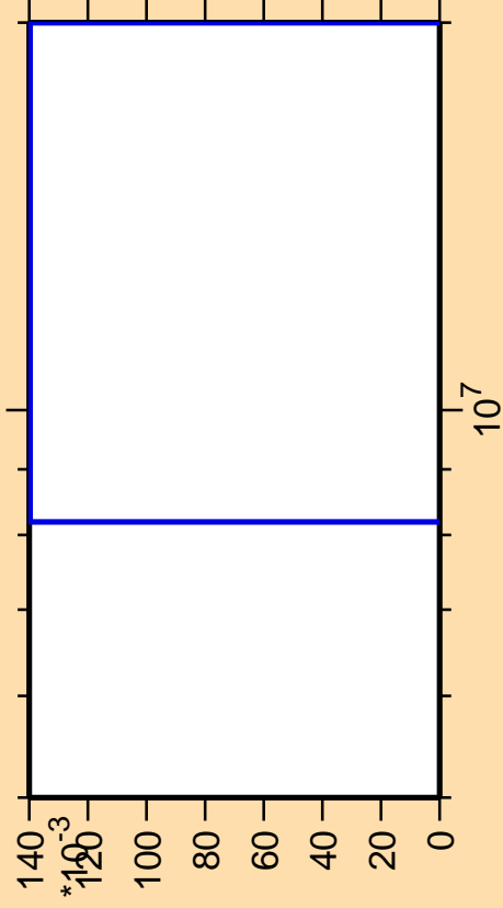
\Delta\sigma/\sigma vs. E for ^{158}\text{Sm}(n,2np)
