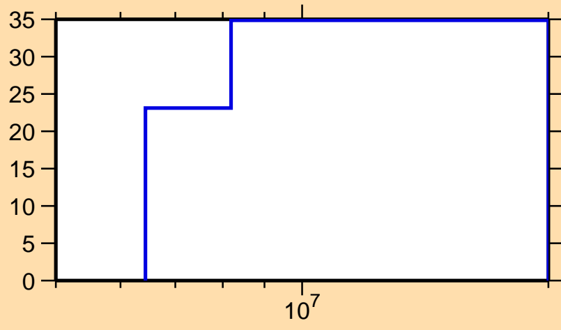
\Delta\sigma/\sigma vs. E for ^{158}\text{Sm}(n,\text{inel.})
