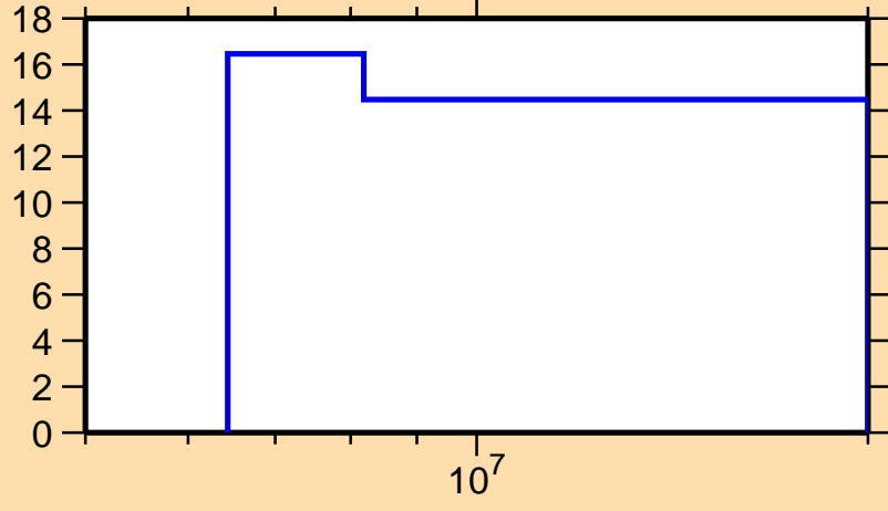
\Delta\sigma/\sigma vs. E for ^{158}\text{Sm}(n,2n)
