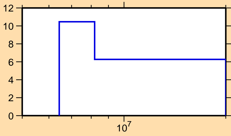
\Delta\sigma/\sigma vs. E for ^{158}\text{Sm}(n,el.)
