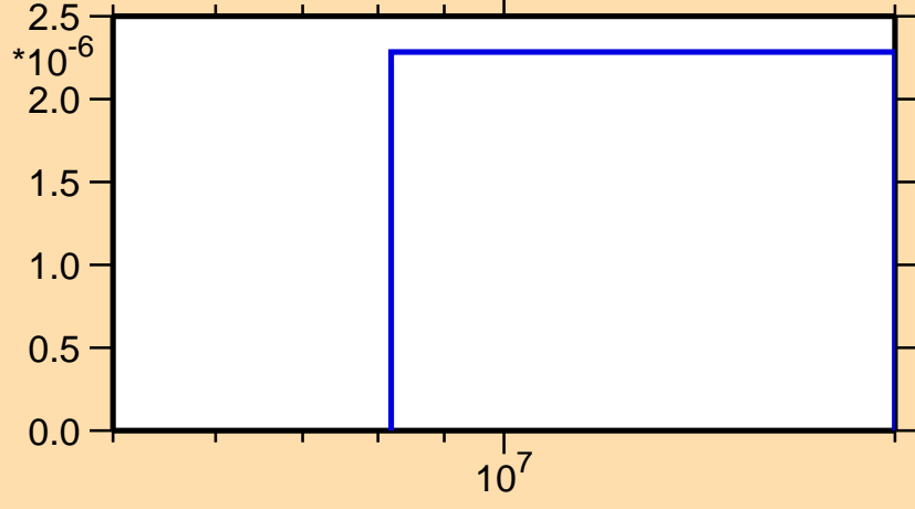
\sigma vs. E for ^{158}\text{Sm}(n,n\alpha)
