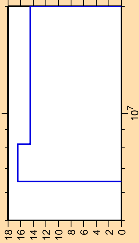
\Delta\sigma/\sigma vs. E for ^{158}\text{Sm}(n,2n)
