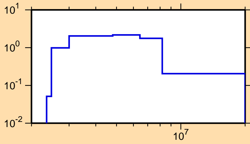
\sigma vs. E for ^{158}\text{Sm}(n,n\text{cont.})
