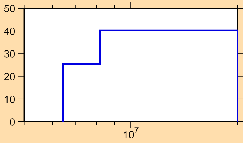
\Delta\sigma/\sigma vs. E for ^{158}\text{Sm}(n,ncont.)
