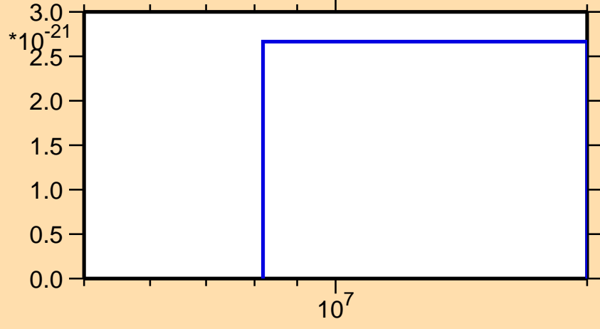
\sigma vs. E for ^{158}\text{Sm}(\text{mt } 11)
