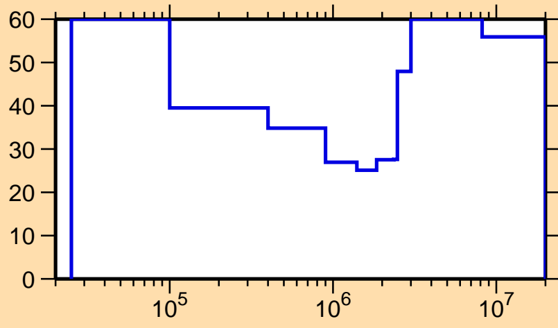
\Delta\sigma/\sigma vs. E for ^{158}\text{Sm}(n,n_1)
