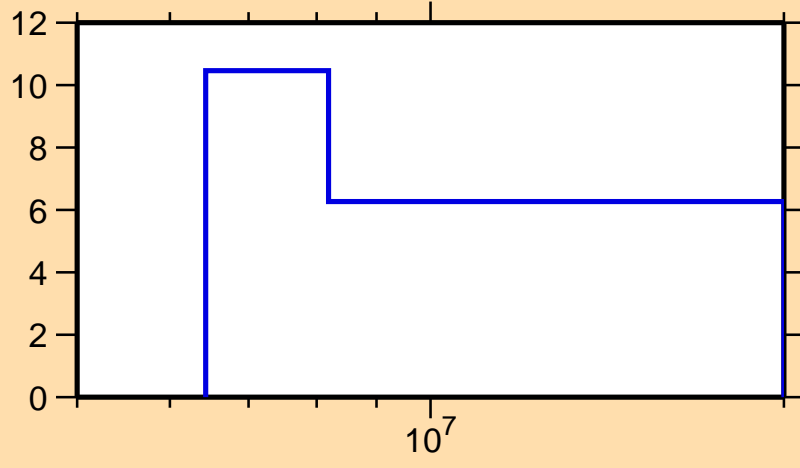
\Delta\sigma/\sigma vs. E for ^{158}\text{Sm}(n,\text{el.})
