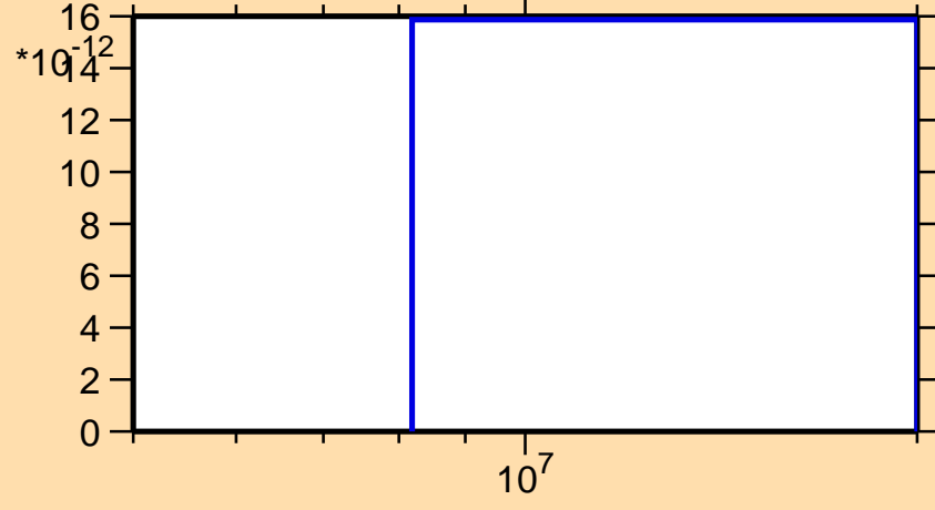
\sigma vs. E for ^{158}\text{Sm}(n,2n\alpha)
