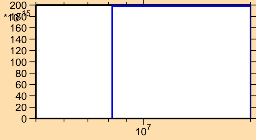
\sigma vs. E for ^{158}\text{Sm}(n,2np)
