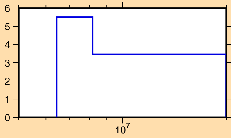
\Delta\sigma/\sigma vs. E for ^{158}\text{Sm}(n,\text{tot.})
