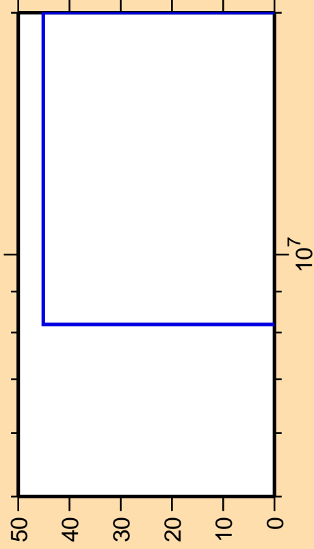
\Delta\sigma/\sigma vs. E for ^{158}\text{Sm}(n,np)
