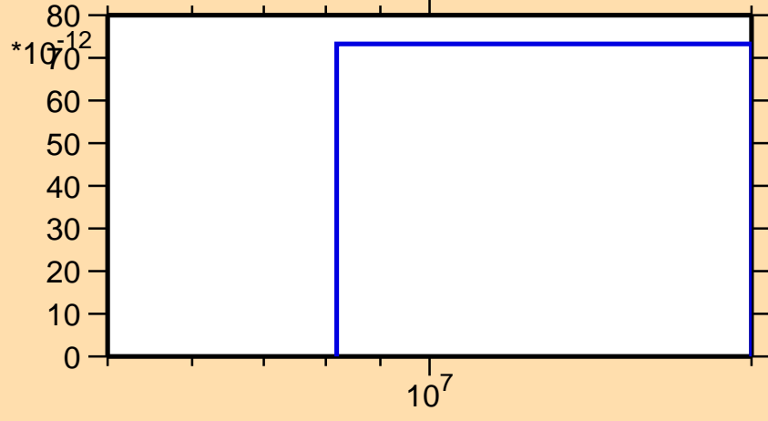
\sigma vs. E for ^{158}\text{Sm}(n,nd)
