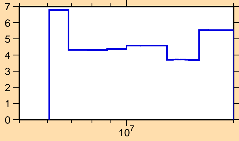
\Delta\sigma/\sigma vs. E for ^{159}\text{Sm}(n,\text{tot.})
