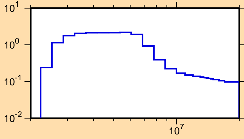
\sigma vs. E for ^{160}\text{Sm}(n,n\text{cont.})
