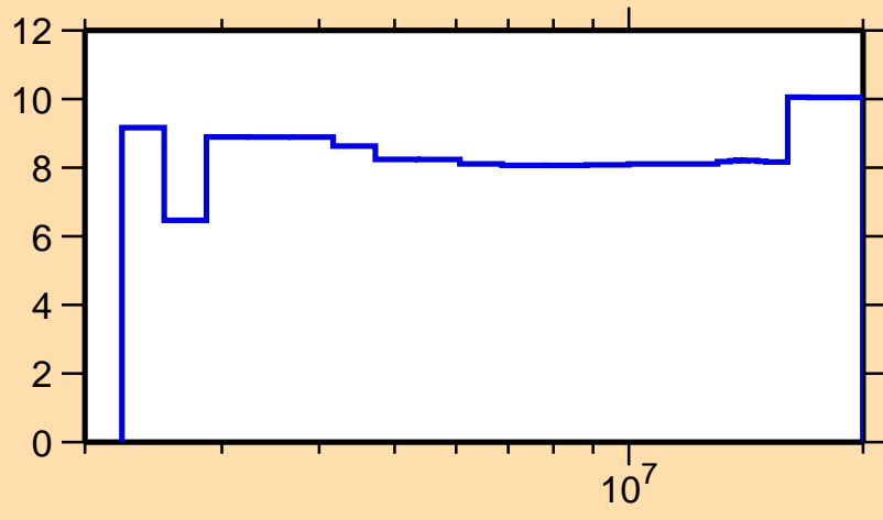
\Delta\sigma/\sigma vs. E for ^{160}\text{Sm}(n,\text{nonel.})
