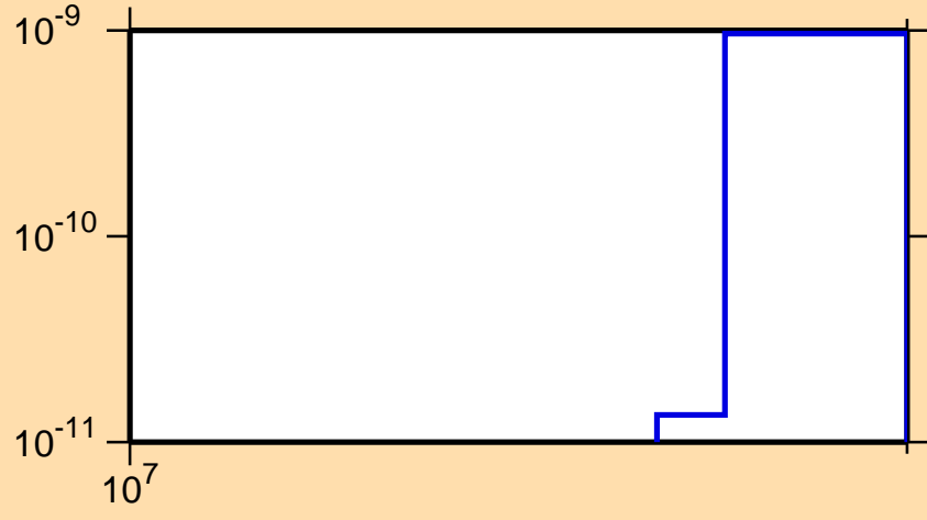
\sigma vs. E for ^{160}\text{Sm}(n,2n\alpha)
