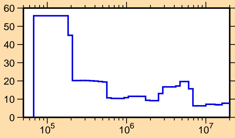
\Delta\sigma/\sigma vs. E for ^{160}\text{Sm}(n,\text{el.})
