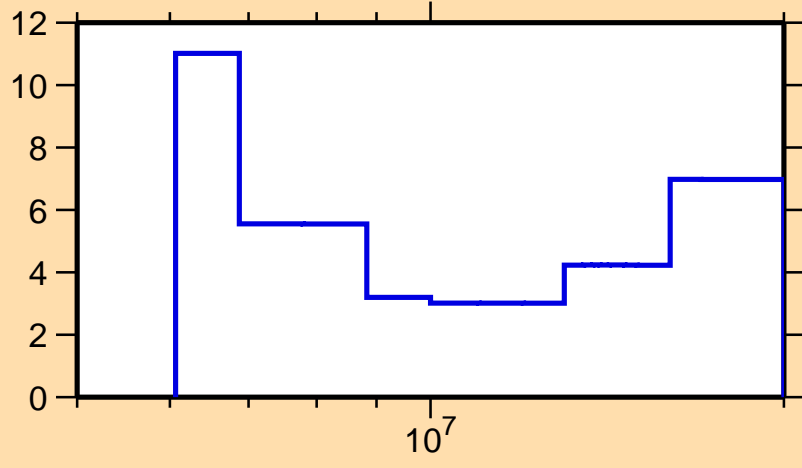
\Delta\sigma/\sigma vs. E for ^{160}\text{Sm}(n,\text{tot.})
