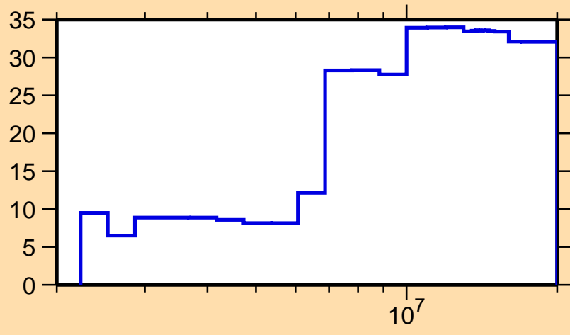
\Delta\sigma/\sigma vs. E for ^{160}\text{Sm}(n,\text{inel.})
