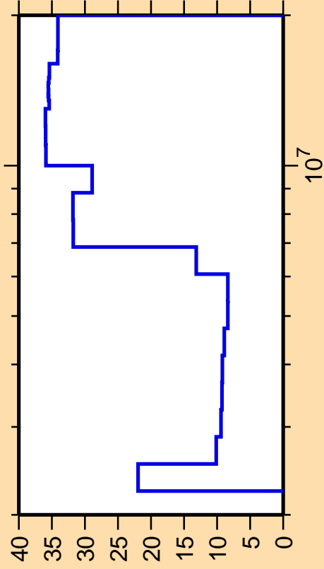
\Delta\sigma/\sigma vs. E for ^{160}\text{Sm}(n,n\text{cont.})
