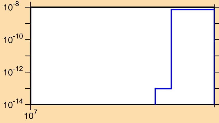
\sigma vs. E for ^{160}\text{Sm}(n,\text{nd})
