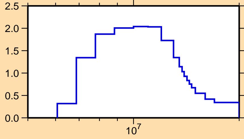
\sigma vs. E for ^{160}\text{Sm}(n,2n)
