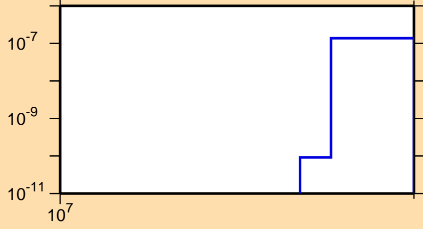
\sigma vs. E for ^{160}\text{Sm}(n,nt)
