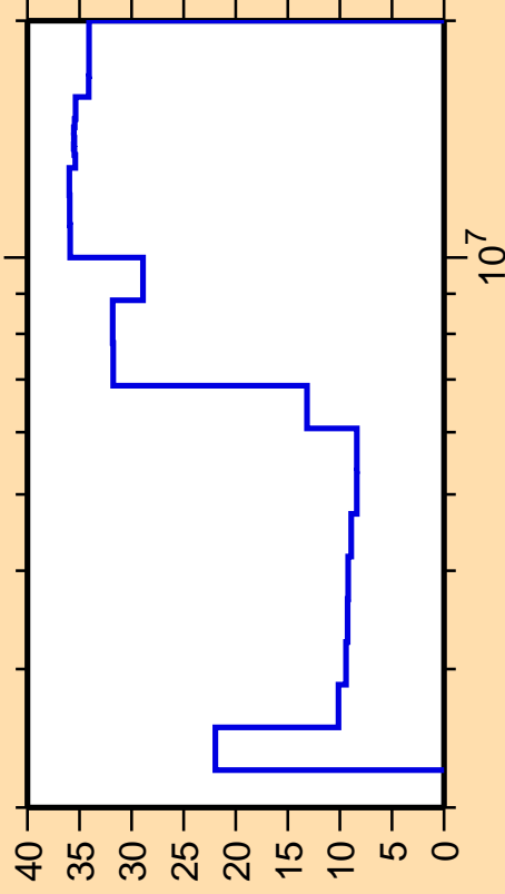
\Delta\sigma/\sigma vs. E for ^{160}\text{Sm}(n,n\text{cont.})
