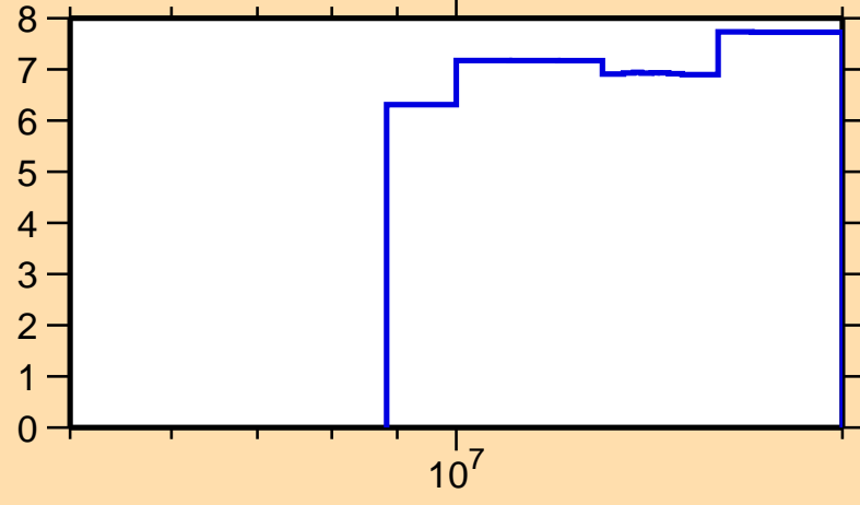
\Delta\sigma/\sigma vs. E for ^{160}\text{Sm}(n,el.)
