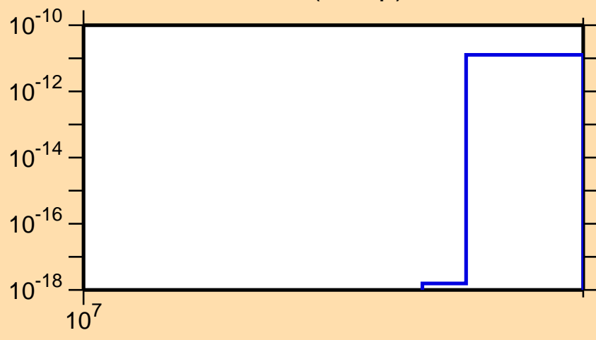
\sigma vs. E for ^{160}\text{Sm}(n,2np)
