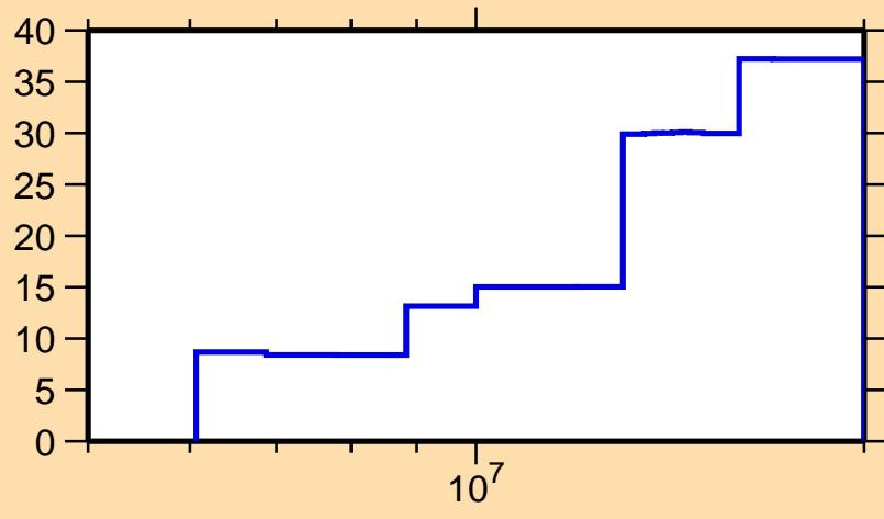
\Delta\sigma/\sigma vs. E for ^{160}\text{Sm}(n,2n)
