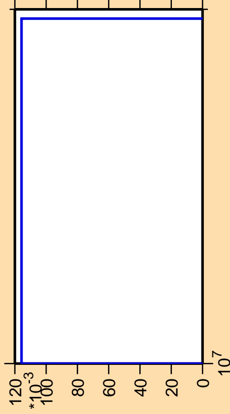
\Delta\sigma/\sigma vs. E for ^{160}\text{Sm}(n,2np)
