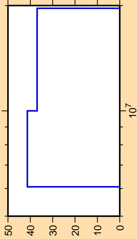
\Delta\sigma/\sigma vs. E for ^{160}\text{Sm}(n,n_1)
