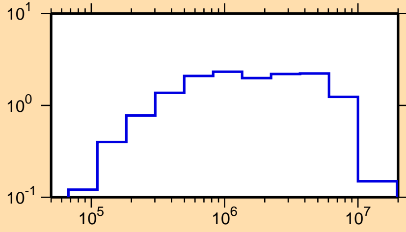
\sigma vs. E for ^{160}\text{Sm}(n,\text{inel.})
