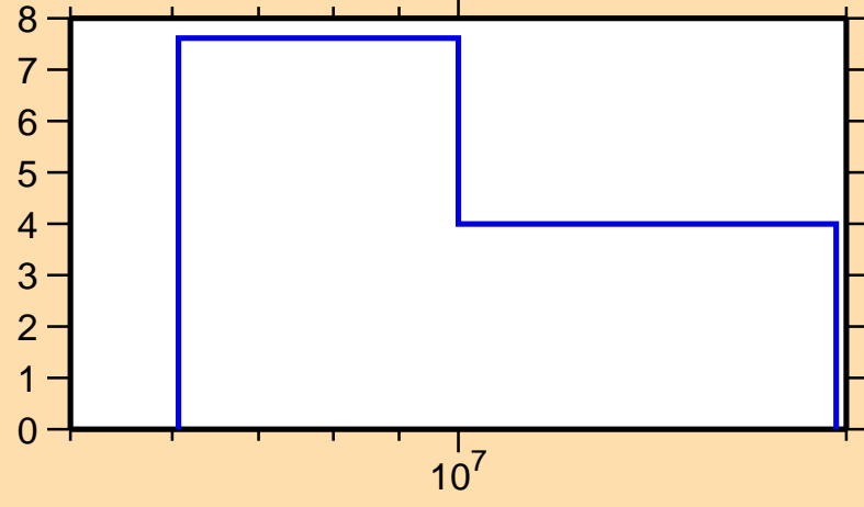
\Delta\sigma/\sigma vs. E for ^{160}\text{Sm}(n,\text{tot.})
