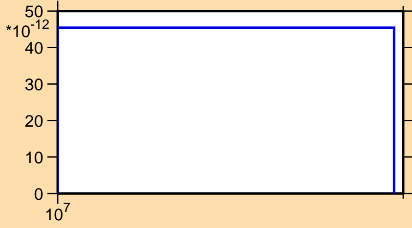
\sigma vs. E for ^{160}\text{Sm}(n,\text{nd})
