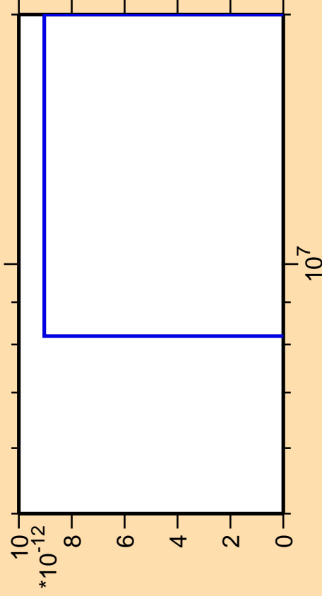
\Delta\sigma/\sigma vs. E for ^{160}\text{Sm}(\text{mt } 11)
