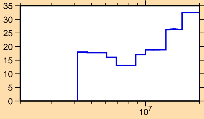
\Delta\sigma/\sigma vs. E for ^{161}\text{Sm}(n,2n)
