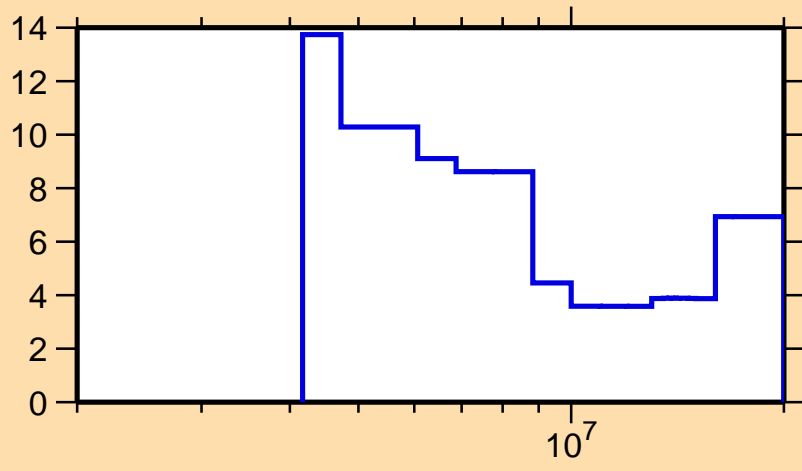
\Delta\sigma/\sigma vs. E for ^{161}\text{Sm}(n,\text{tot.})
