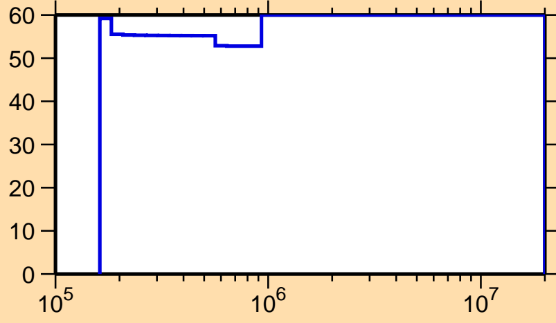
\Delta\sigma/\sigma vs. E for ^{161}\text{Sm}(n,n_1)
