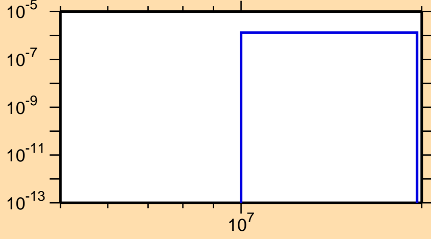
\sigma vs. E for ^{161}\text{Sm}(n,n\alpha)
