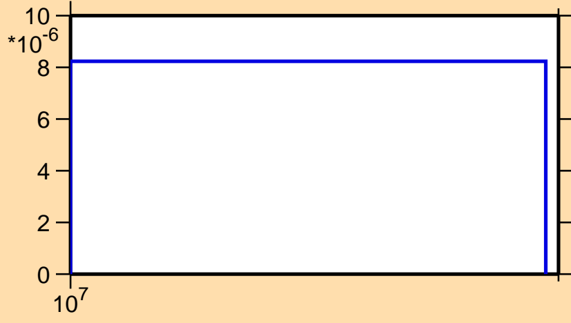
\sigma vs. E for ^{161}\text{Sm}(n,d)
