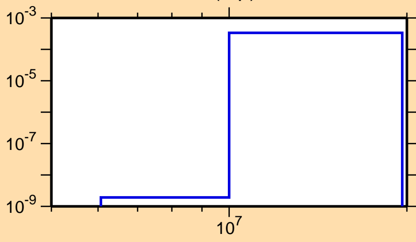
\sigma vs. E for ^{161}\text{Sm}(n,p)
