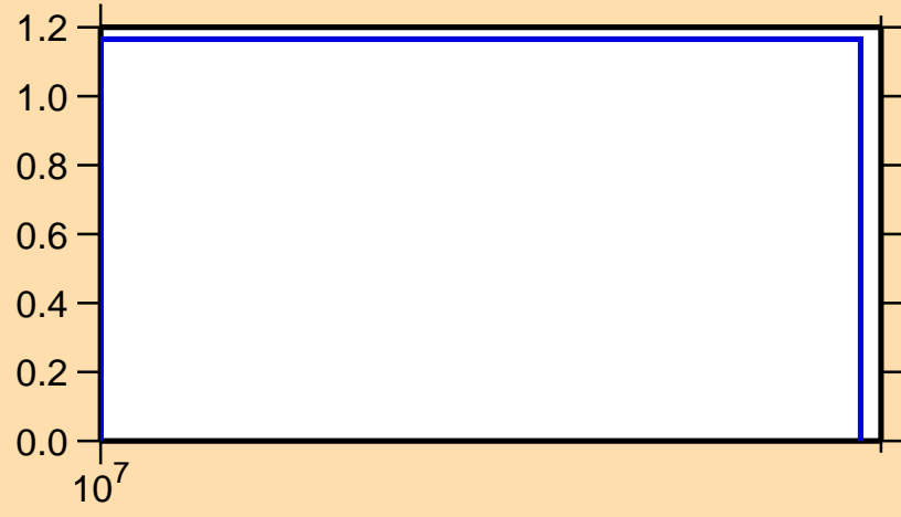
\sigma vs. E for ^{161}\text{Sm}(n,3n)
