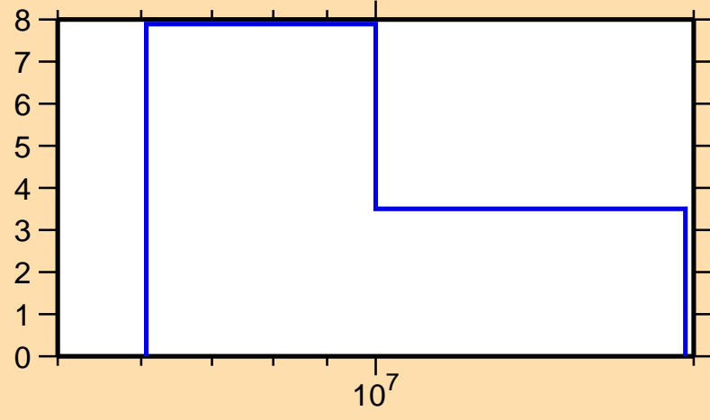
\Delta\sigma/\sigma vs. E for ^{161}\text{Sm}(n,\text{tot.})
