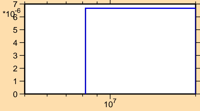
\sigma vs. E for ^{161}\text{Sm}(n,d)
