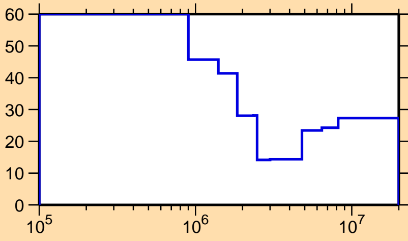
\Delta\sigma/\sigma vs. E for ^{161}\text{Sm}(n,n\text{cont.})
