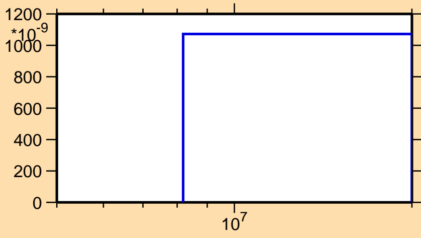
\sigma vs. E for ^{161}\text{Sm}(n,n\alpha)
