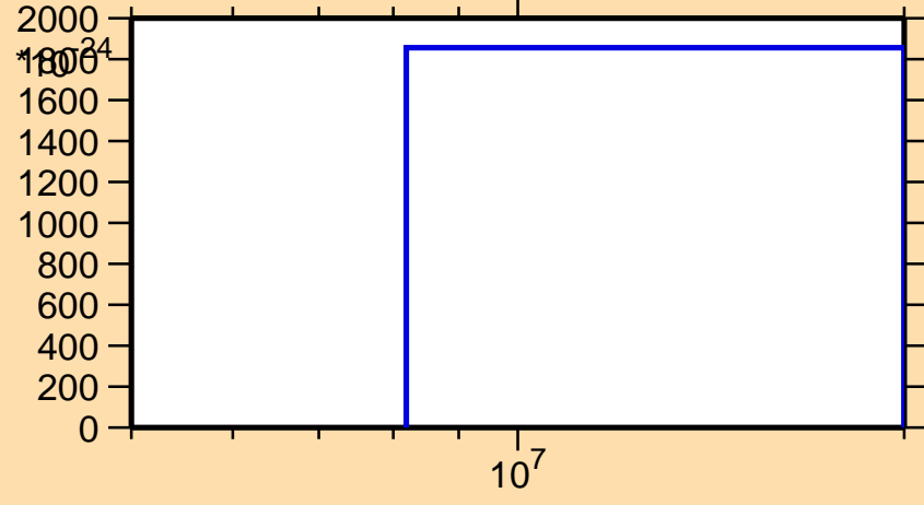
\sigma vs. E for ^{161}\text{Sm} (mt 11)
