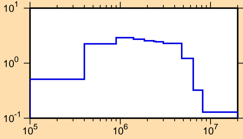
\sigma vs. E for ^{161}\text{Sm}(n,\text{inel.})
