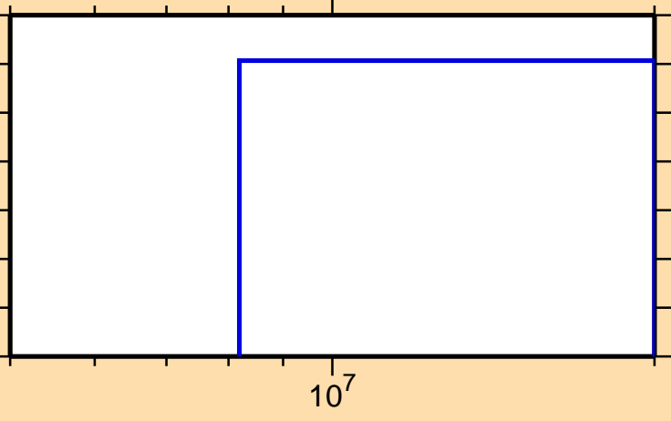
\sigma vs. E for ^{161}\text{Sm}(n,nt)
