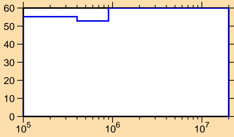
\Delta\sigma/\sigma vs. E for ^{161}\text{Sm}(n,n_1)
