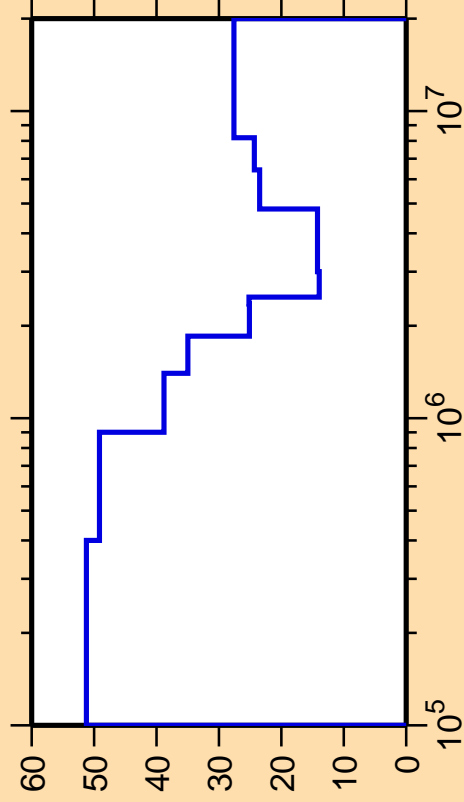
\Delta\sigma/\sigma vs. E for ^{161}\text{Sm}(n,\text{inel.})
