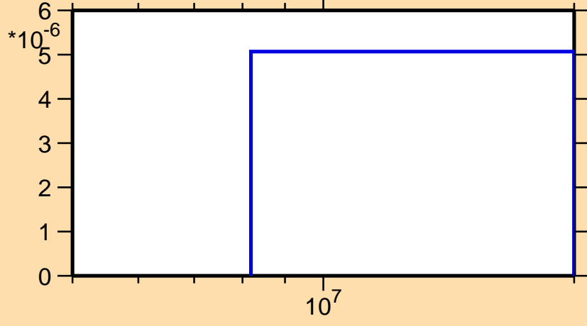
\sigma vs. E for ^{161}\text{Sm}(n,t)
