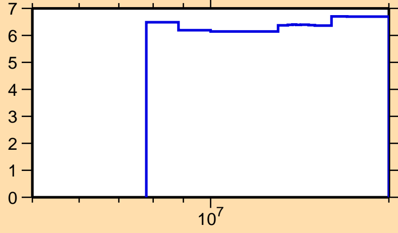
\Delta\sigma/\sigma vs. E for ^{162}\text{Sm}(n,\text{nonel.})
