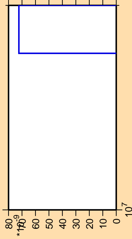
\Delta\sigma/\sigma vs. E for ^{162}\text{Sm} (mt 11)
