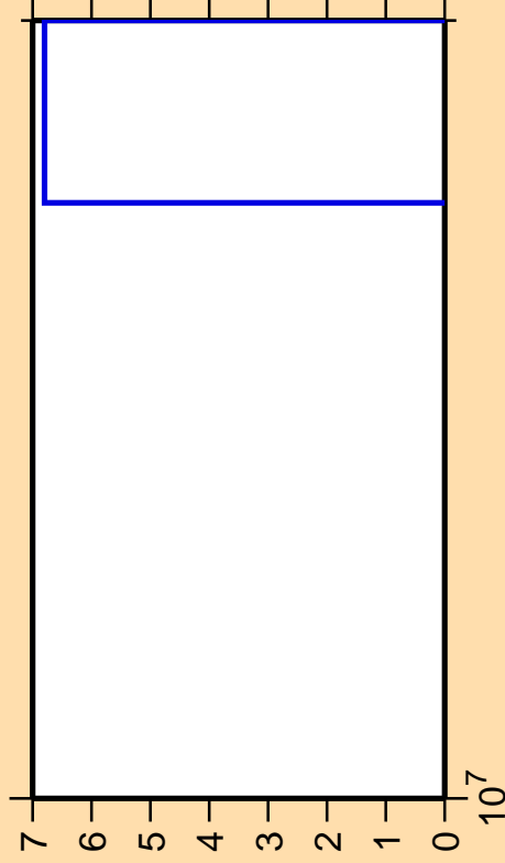
\Delta\sigma/\sigma vs. E for ^{162}\text{Sm}(n,2np)
