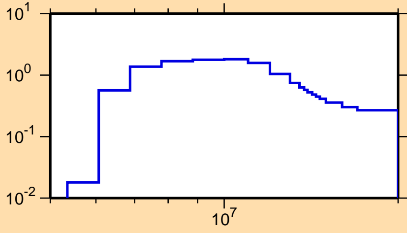
\sigma vs. E for ^{162}\text{Sm}(n,2n)
