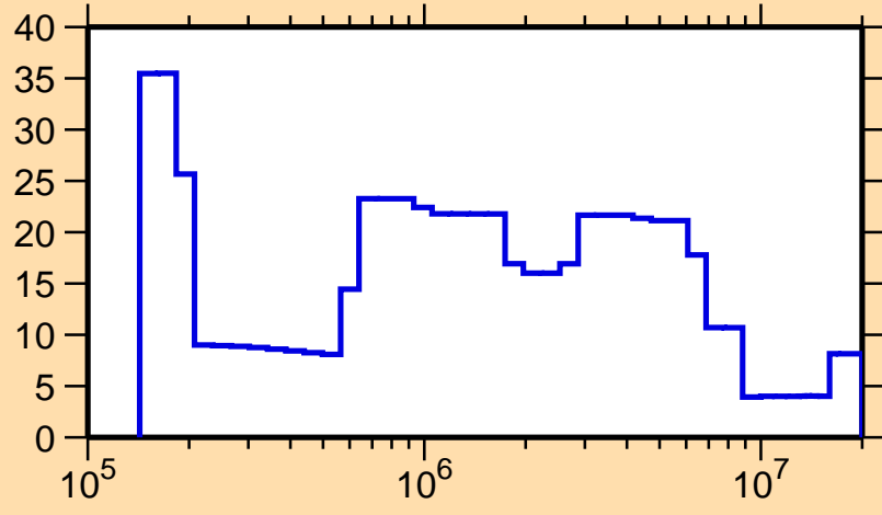
\Delta\sigma/\sigma vs. E for ^{163}\text{Sm}(n,\text{tot.})
