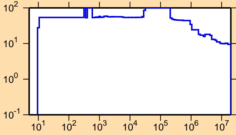
\Delta\sigma/\sigma vs. E for ^{163}\text{Sm}(n,\text{nonel.})
