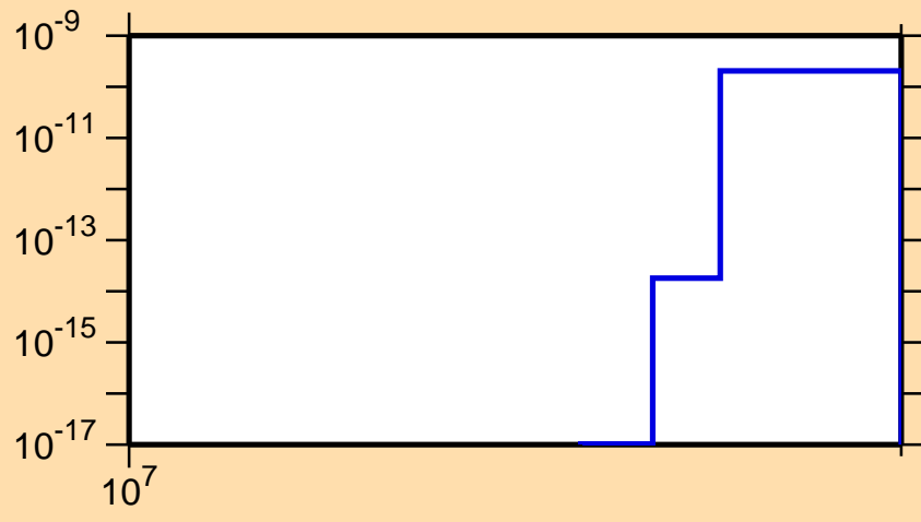
\sigma vs. E for ^{163}\text{Sm}(n,2np)
