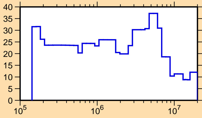
\Delta\sigma/\sigma vs. E for ^{163}\text{Sm}(n, el.)
