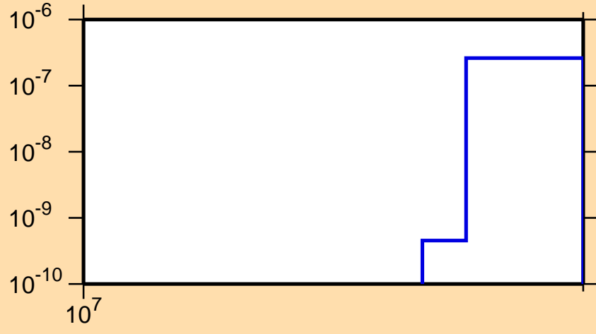
\sigma vs. E for ^{163}\text{Sm}(n,nt)
