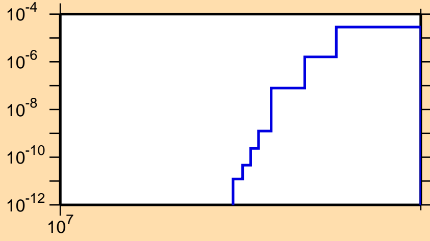
\sigma vs. E for ^{163}\text{Sm}(n,np)
