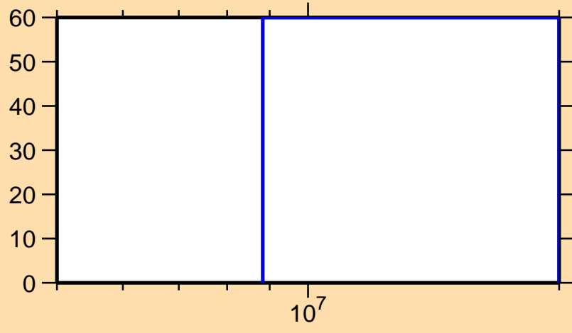
\Delta\sigma/\sigma vs. E for ^{163}\text{Sm}(n,ncont.)
