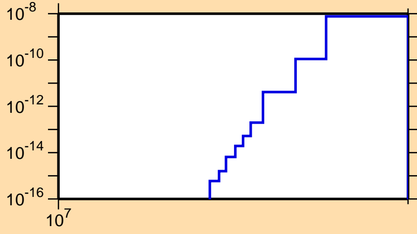
\sigma vs. E for ^{163}\text{Sm}(n,2n\alpha)
