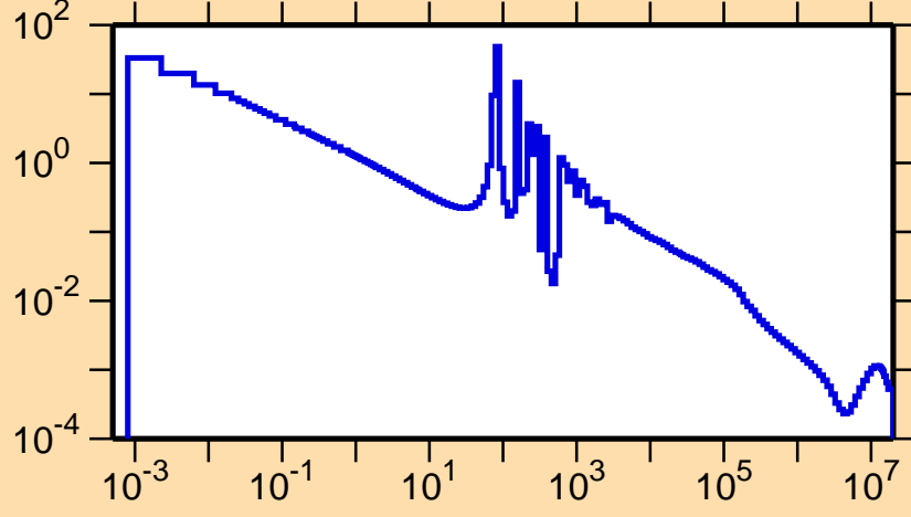
\sigma vs. E for ^{163}\text{Sm}(n,\gamma)
