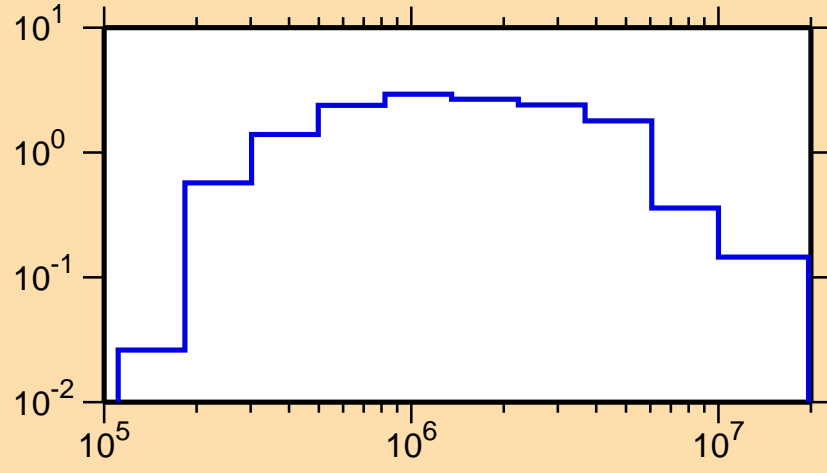
\sigma vs. E for ^{163}\text{Sm}(n,\text{inel.})
