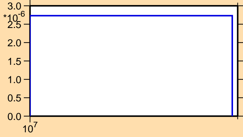
\sigma vs. E for ^{163}\text{Sm}(n,d)
