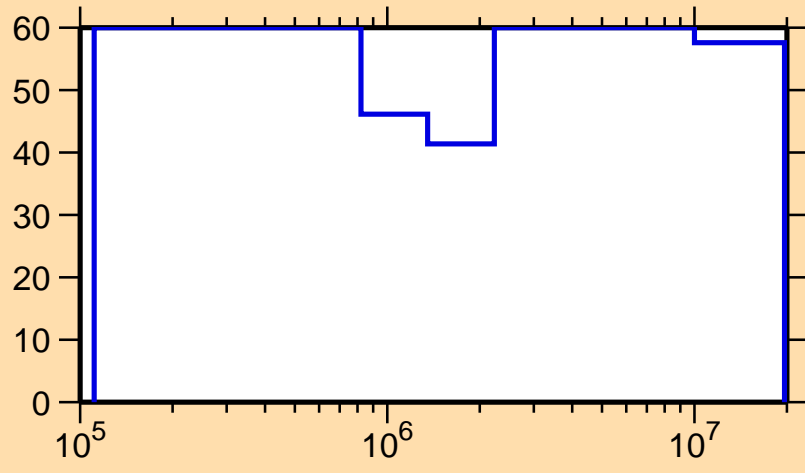
\Delta\sigma/\sigma vs. E for ^{163}\text{Sm}(n,n_1)
