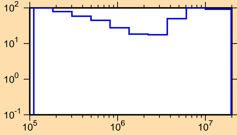
\Delta\sigma/\sigma vs. E for ^{163}\text{Sm}(n,n\text{cont.})
