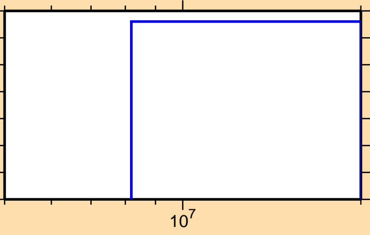
\sigma vs. E for ^{163}\text{Sm} (mt 11)
