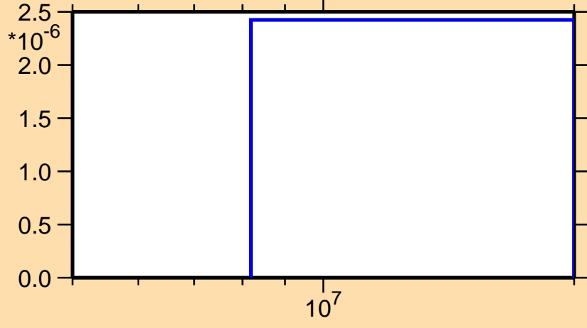
\sigma vs. E for ^{163}\text{Sm}(n,t)
