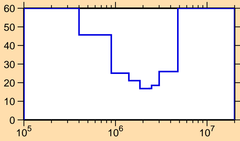
\Delta\sigma/\sigma vs. E for ^{163}\text{Sm}(n,n\text{cont.})
