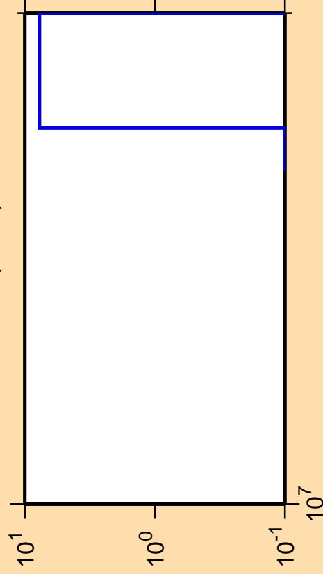
\Delta\sigma/\sigma vs. E for ^{100}\text{Sn}(n,nd)
