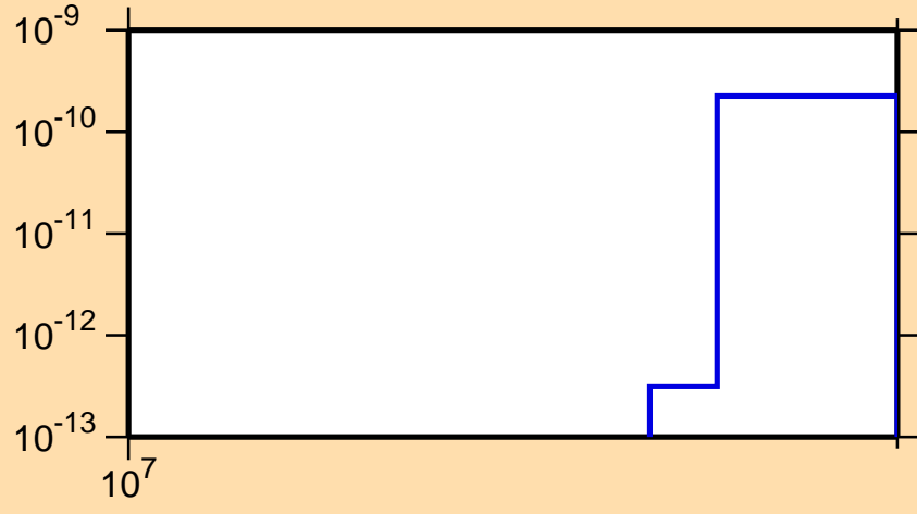
\sigma vs. E for ^{100}\text{Sn}(\text{mt } 34)
