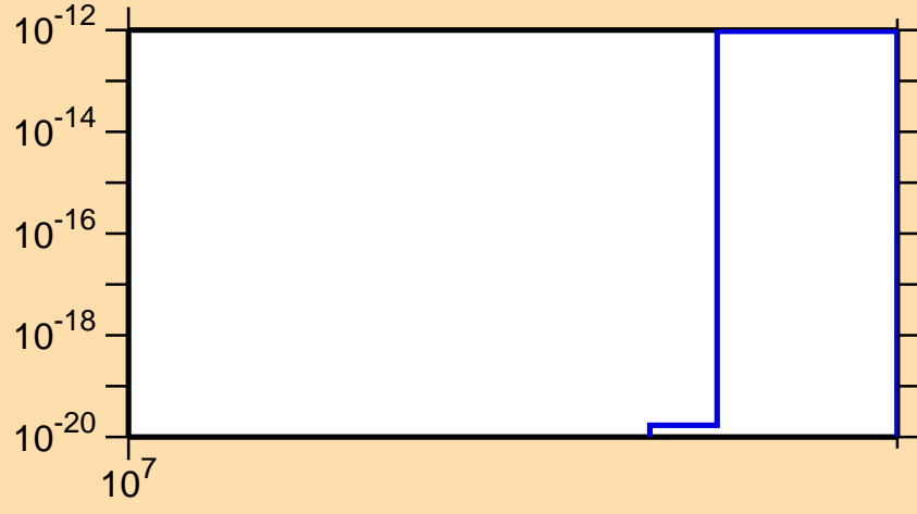
\sigma vs. E for ^{100}\text{Sn}(n,nd)
