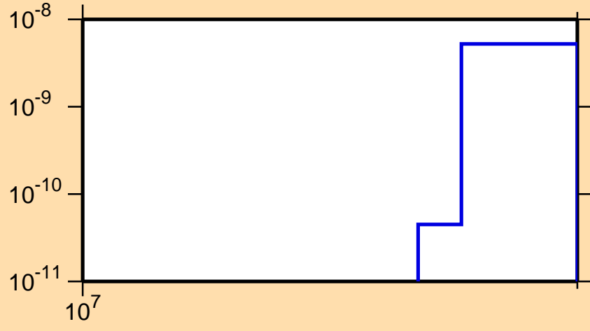
\sigma vs. E for ^{100}\text{Sn}(\text{mt } 45)
