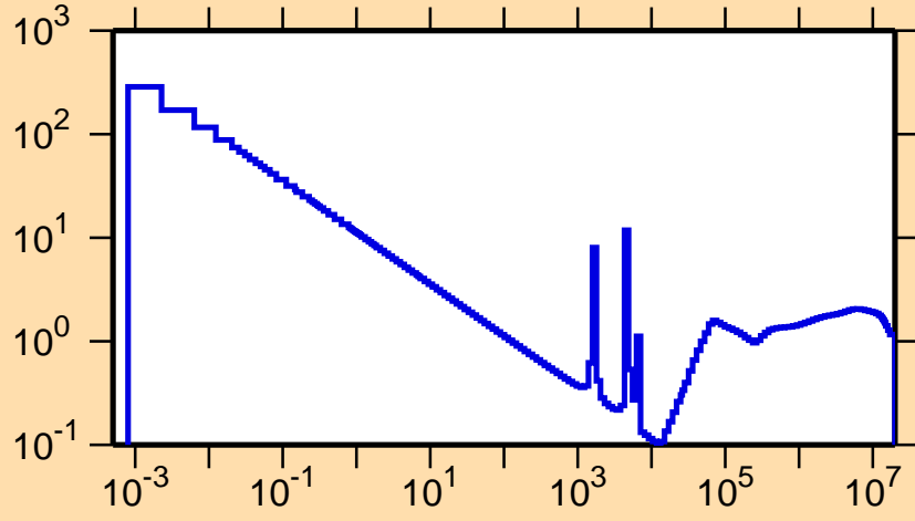
\sigma vs. E for ^{100}\text{Sn}(n,\text{nonel.})
