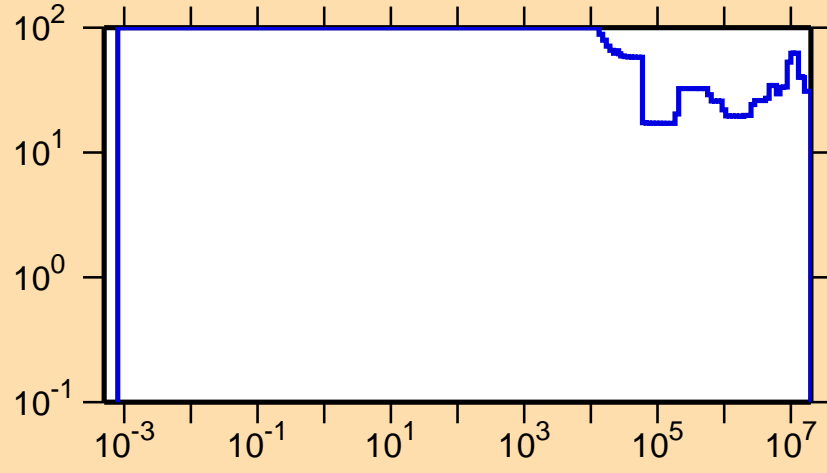
\Delta\sigma/\sigma vs. E for ^{100}\text{Sn}(n,p)
