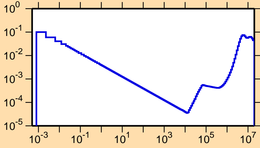
\sigma vs. E for ^{100}\text{Sn}(n,\alpha)
