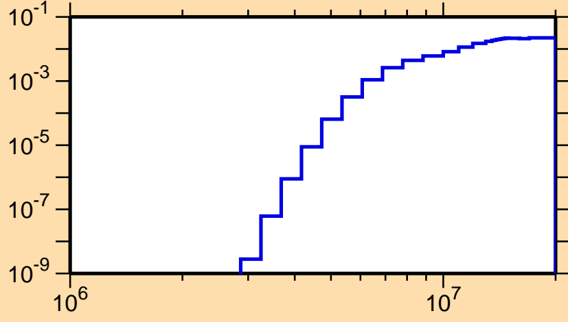
\sigma vs. E for ^{100}\text{Sn}(n,d)
