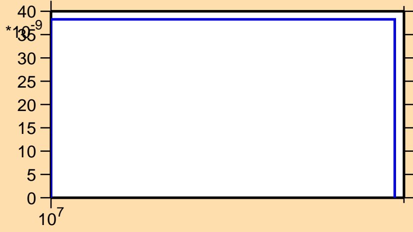
\sigma vs. E for ^{100}\text{Sn}(n,\text{pt})
