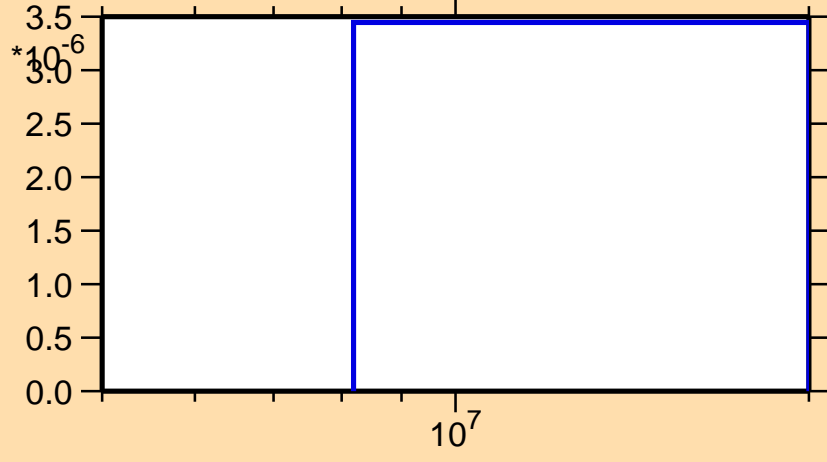
\sigma vs. E for ^{100}\text{Sn}(n,n\alpha)
