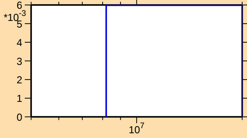
\sigma vs. E for ^{101}\text{Sn}(n,2n)
