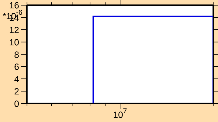
\sigma vs. E for ^{101}\text{Sn}(n,\text{pt})
