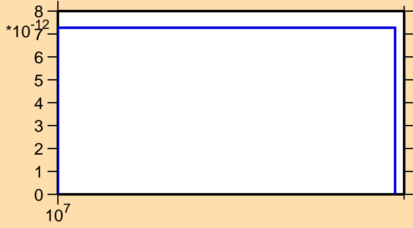
\sigma vs. E for ^{104}\text{Sn} (mt 34)
