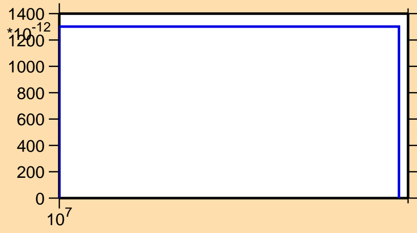
\sigma vs. E for ^{104}\text{Sn}(n,2np)
