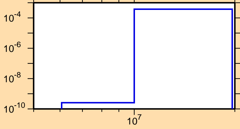
\sigma vs. E for ^{104}\text{Sn}(n,\text{pd})
