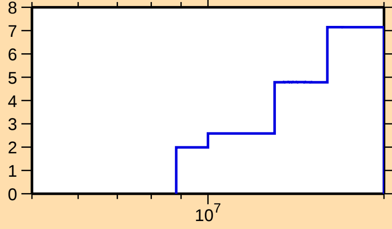
\Delta\sigma/\sigma vs. E for ^{105}\text{Sn}(n,\text{tot.})
