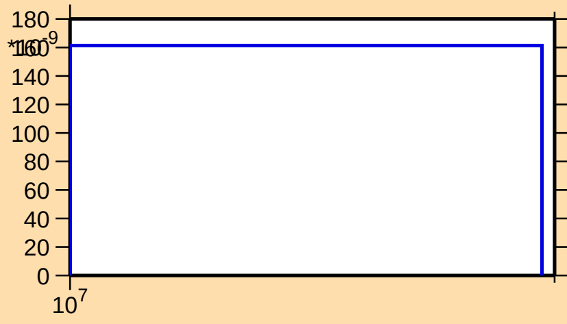
\sigma vs. E for ^{105}\text{Sn}(n,\text{nd})
