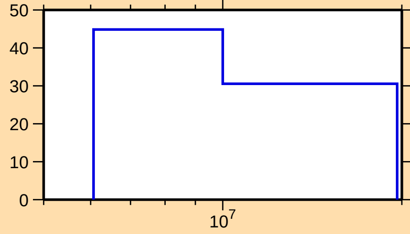
\Delta\sigma/\sigma vs. E for ^{105}\text{Sn}(n,\text{inel.})
