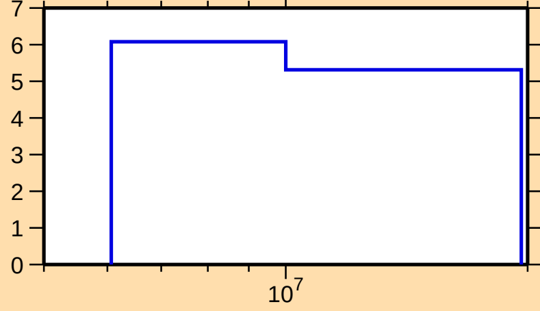
\Delta\sigma/\sigma vs. E for ^{105}\text{Sn}(n,\text{nonel.})
