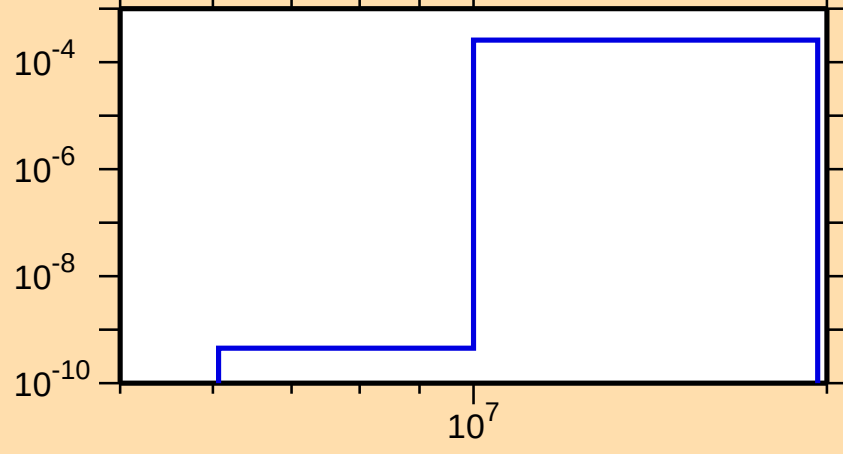
\sigma vs. E for ^{105}\text{Sn}(n,t)
