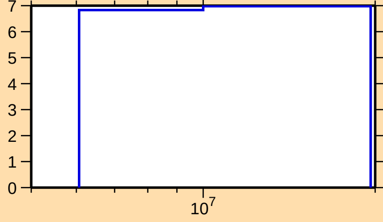
\Delta\sigma/\sigma vs. E for ^{105}\text{Sn}(n,\text{el.})
