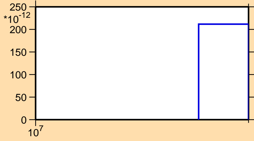
\sigma vs. E for ^{106}\text{Sn} (mt 34)
