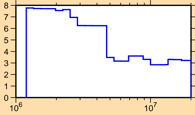
\Delta\sigma/\sigma vs. E for ^{106}\text{Sn}(n,\text{nonel.})
