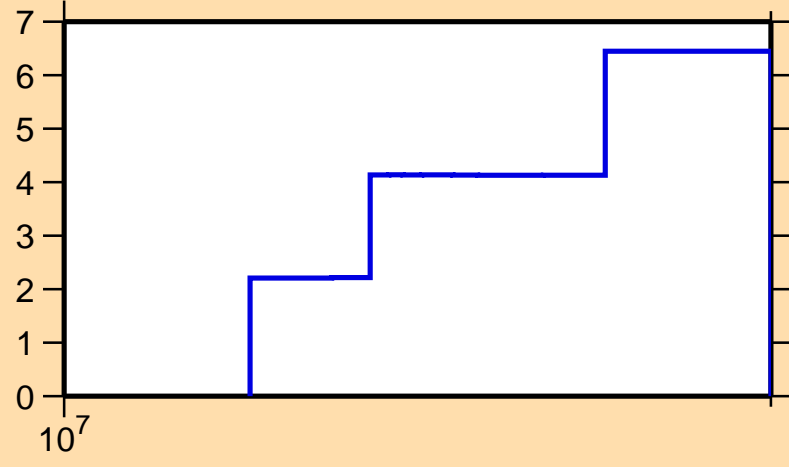
\Delta\sigma/\sigma vs. E for ^{106}\text{Sn}(n,\text{tot.})
