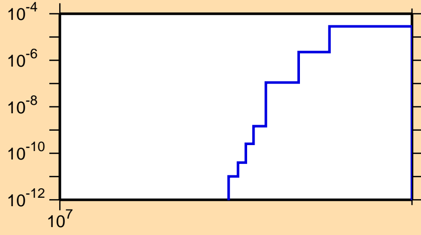
\sigma vs. E for ^{107}\text{Sn}(n,nd)
