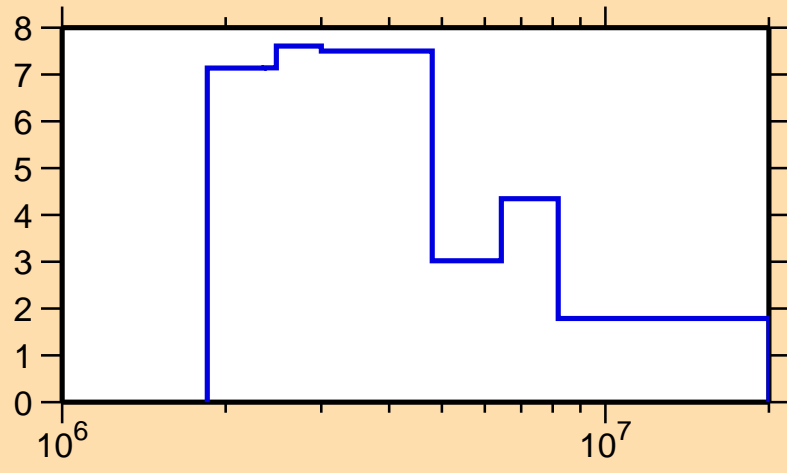
\Delta\sigma/\sigma vs. E for ^{107}\text{Sn}(n,\text{el.})
