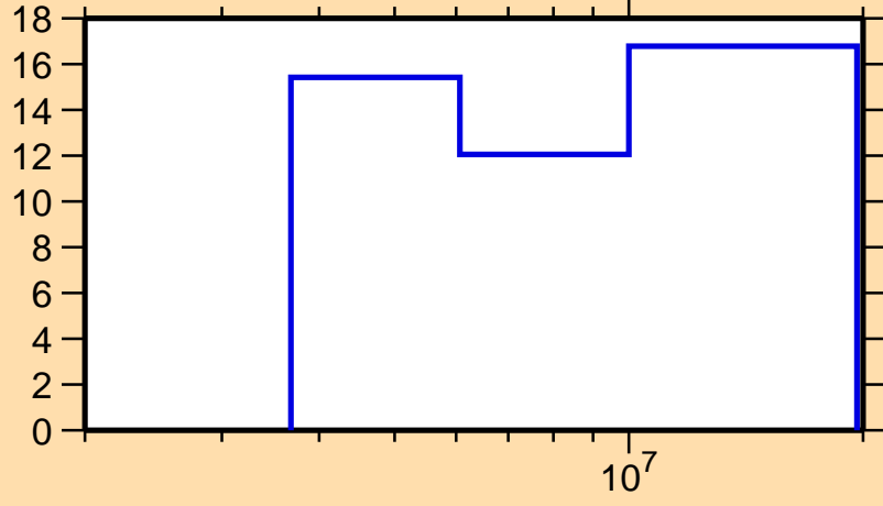
\Delta\sigma/\sigma vs. E for ^{108}\text{Sn}(n,n\text{cont.})
