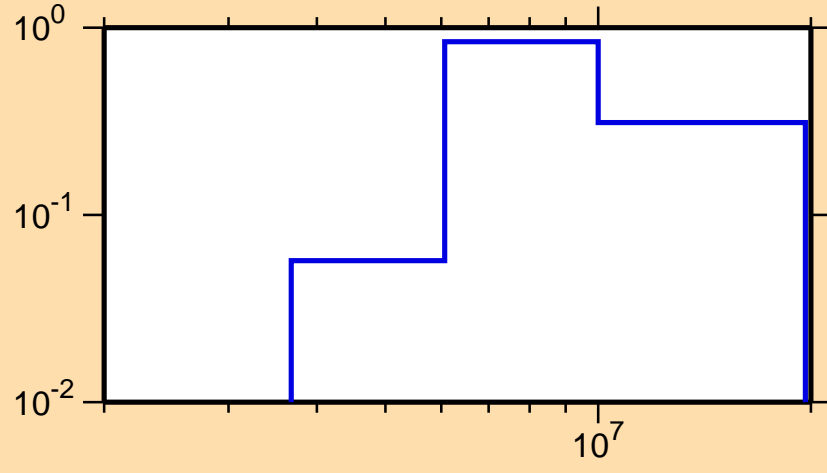
\sigma vs. E for ^{108}\text{Sn}(n,n\text{cont.})
