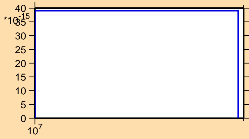
\sigma vs. E for ^{108}\text{Sn} (mt 34)
