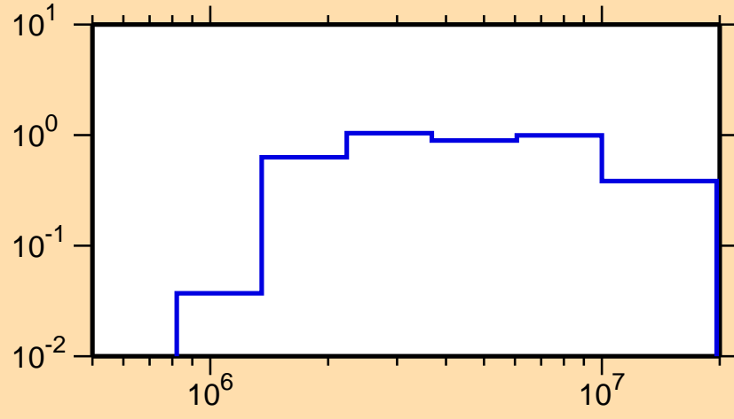
\sigma vs. E for ^{108}\text{Sn}(n,\text{inel.})
