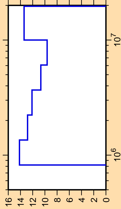
\Delta\sigma/\sigma vs. E for ^{108}\text{Sn}(n,\text{inel.})
