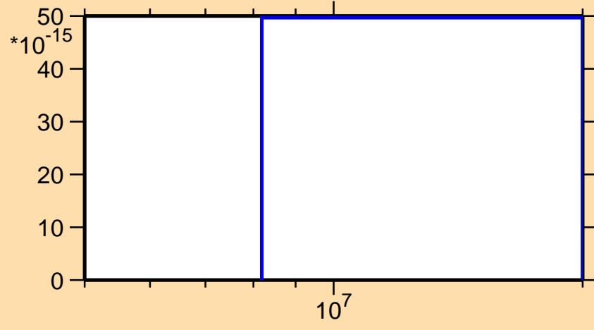
\sigma vs. E for ^{108}\text{Sn}(\text{mt } 34)
