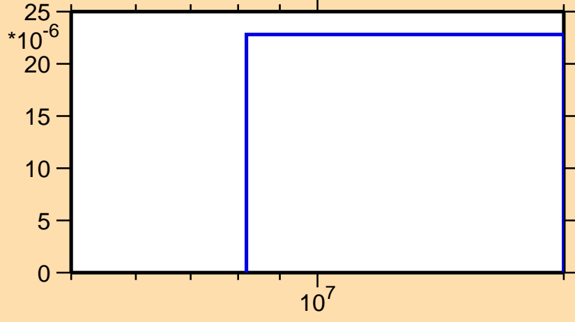
\sigma vs. E for ^{108}\text{Sn}(n,t)
