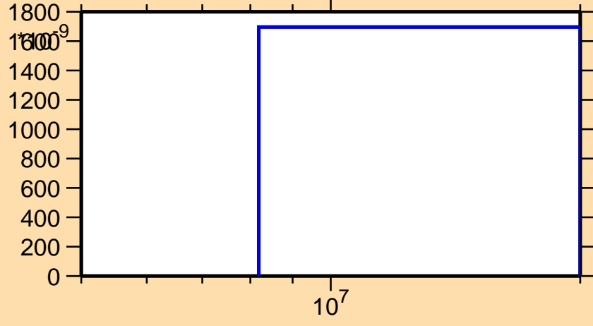
\sigma vs. E for ^{108}\text{Sn}(n,pd)
