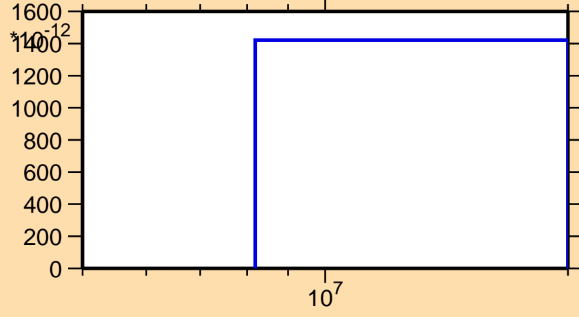
\sigma vs. E for ^{108}\text{Sn}(\text{mt } 45)
