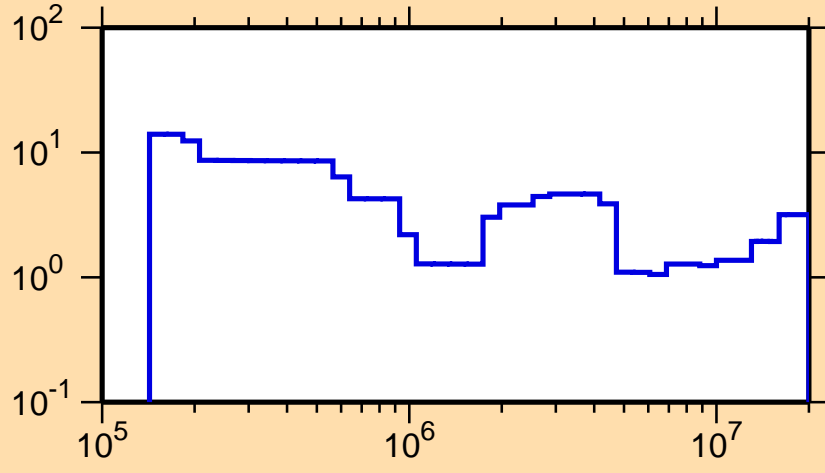
\Delta\sigma/\sigma vs. E for ^{111}\text{Sn}(n,\text{tot.})
