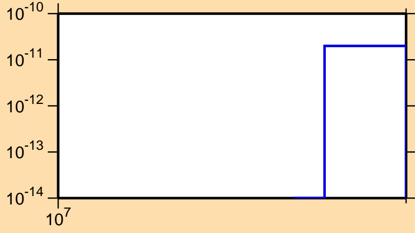
\sigma vs. E for ^{111}\text{Sn} (mt 34)
