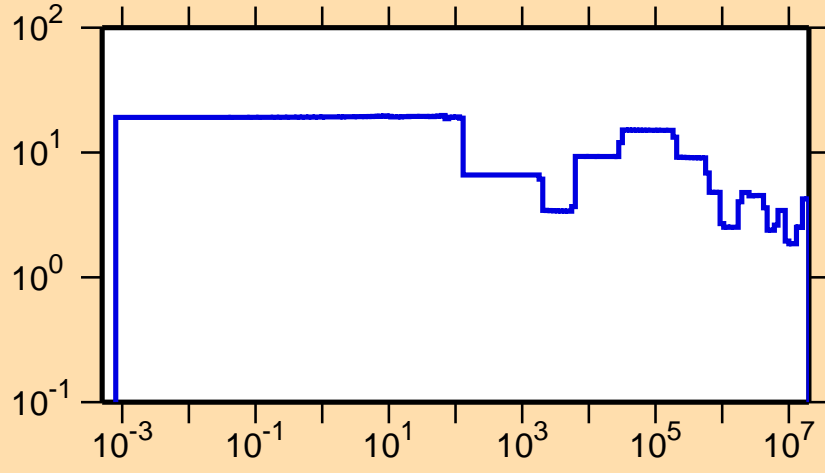
\Delta\sigma/\sigma vs. E for ^{111}\text{Sn}(n,\text{el.})
