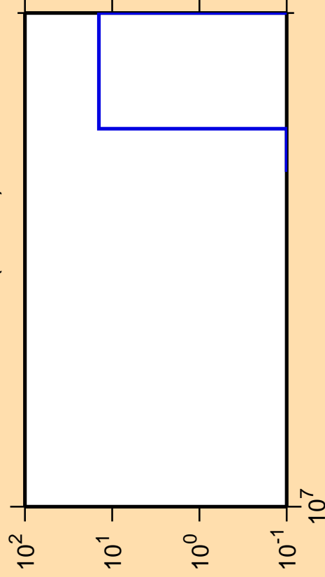
\Delta\sigma/\sigma vs. E for ^{111}\text{Sn}(\text{mt } 45)
