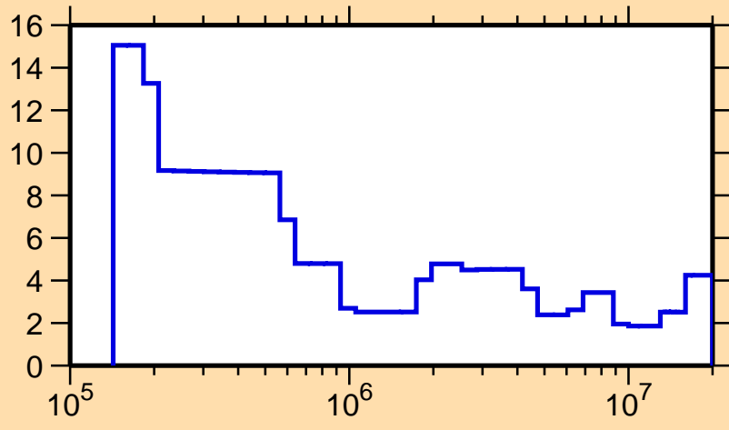
\Delta\sigma/\sigma vs. E for ^{111}\text{Sn}(n,\text{el.})
