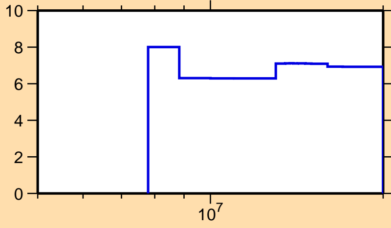
\Delta\sigma/\sigma vs. E for ^{111}\text{Sn}(n,2n)
