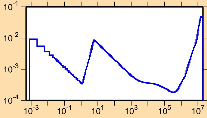
\sigma vs. E for ^{111}\text{Sn}(n,\alpha)
