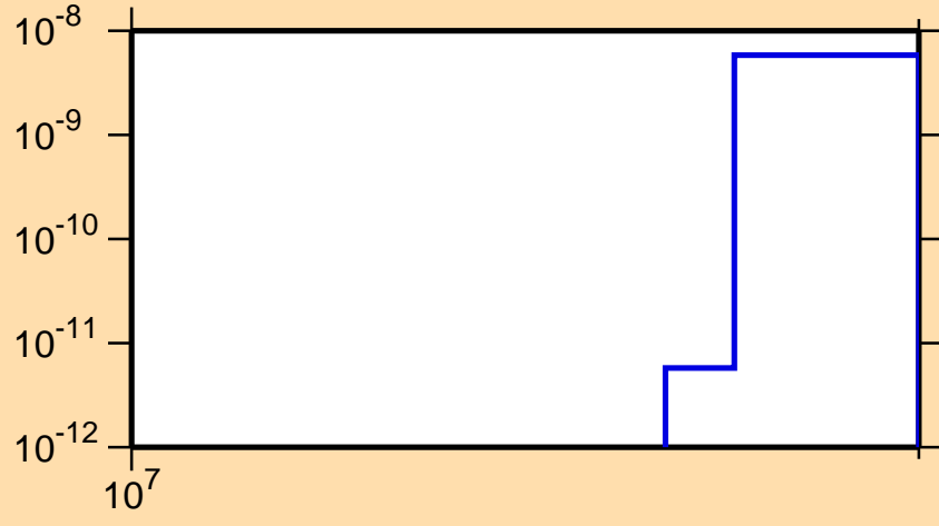
\sigma vs. E for ^{111}\text{Sn}(n,\text{pt})
