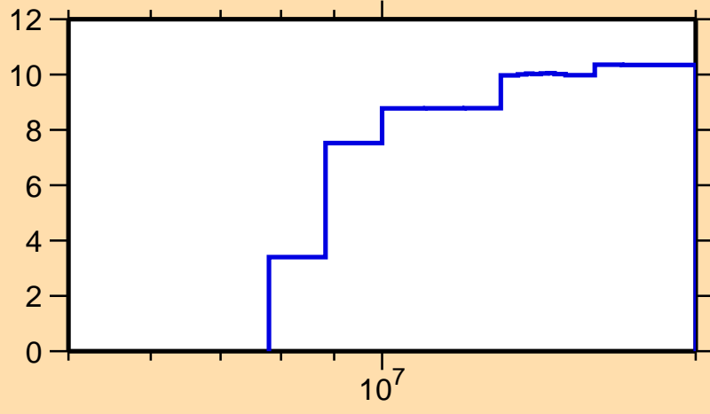
\Delta\sigma/\sigma vs. E for ^{111}\text{Sn}(n,\text{inel.})
