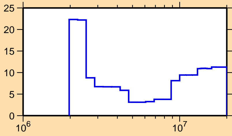
\Delta\sigma/\sigma vs. E for ^{111}\text{Sn}(n,n\text{cont.})
