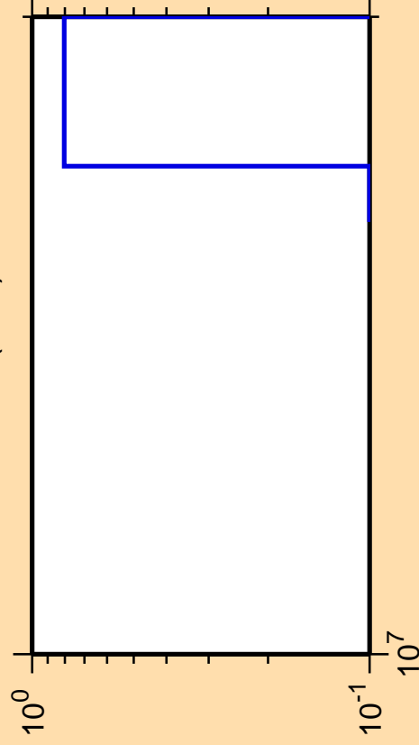
\Delta\sigma/\sigma vs. E for ^{111}\text{Sn}(n,nt)
