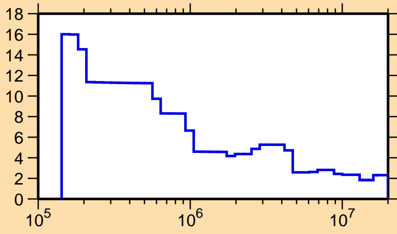
\Delta\sigma/\sigma vs. E for ^{111}\text{Sn}(n,\text{nonel.})
