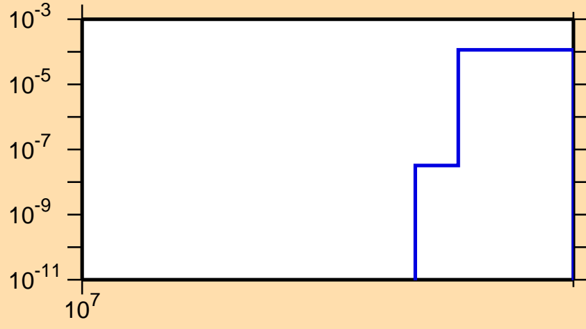
\sigma vs. E for ^{111}\text{Sn}(n,2np)
