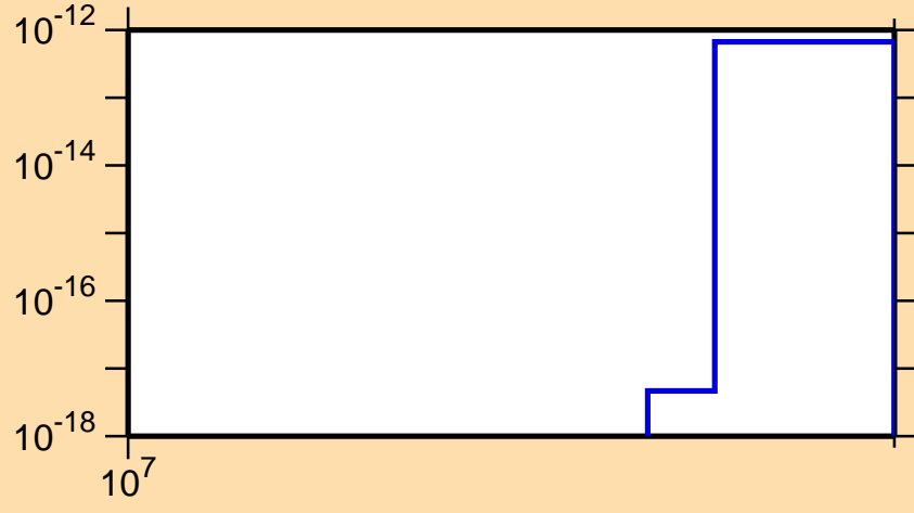
\sigma vs. E for ^{111}\text{Sn}(n,nt)
