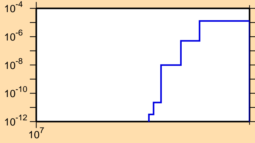
\sigma vs. E for ^{111}\text{Sn}(n,\text{nd})
