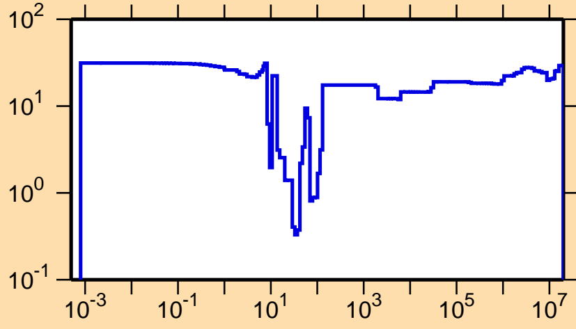
\Delta\sigma/\sigma vs. E for ^{111}\text{Sn}(n,\gamma)
