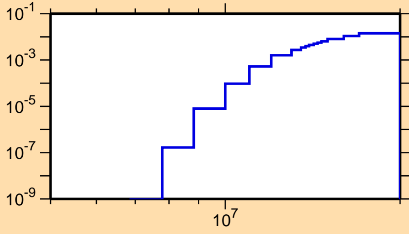
\sigma vs. E for ^{111}\text{Sn}(n,d)
