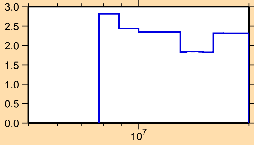
\Delta\sigma/\sigma vs. E for ^{111}\text{Sn}(n,\text{nonel.})
