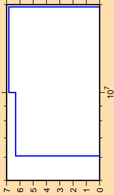
\Delta\sigma/\sigma vs. E for ^{111}\text{Sn}(n,2n)
