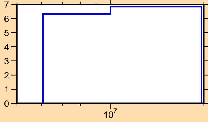
\Delta\sigma/\sigma vs. E for ^{111}\text{Sn}(n,2n)
