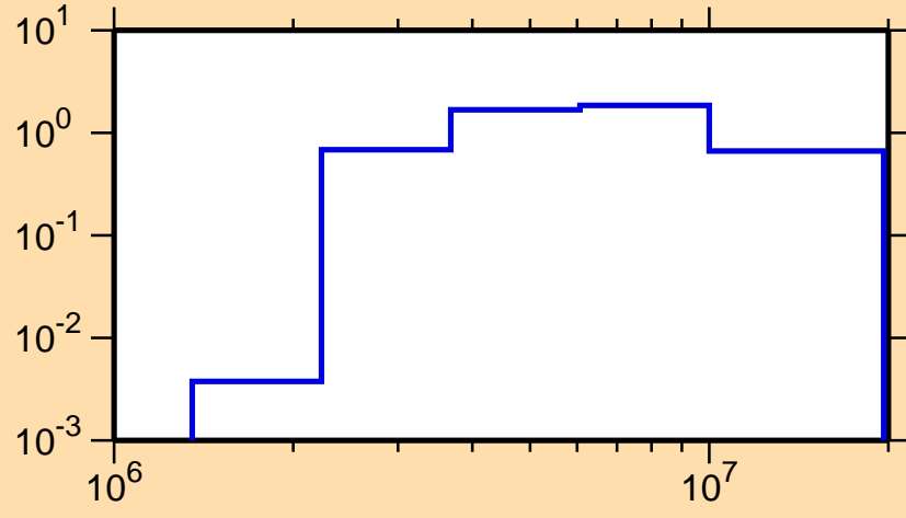
\sigma vs. E for ^{111}\text{Sn}(n,n\text{cont.})
