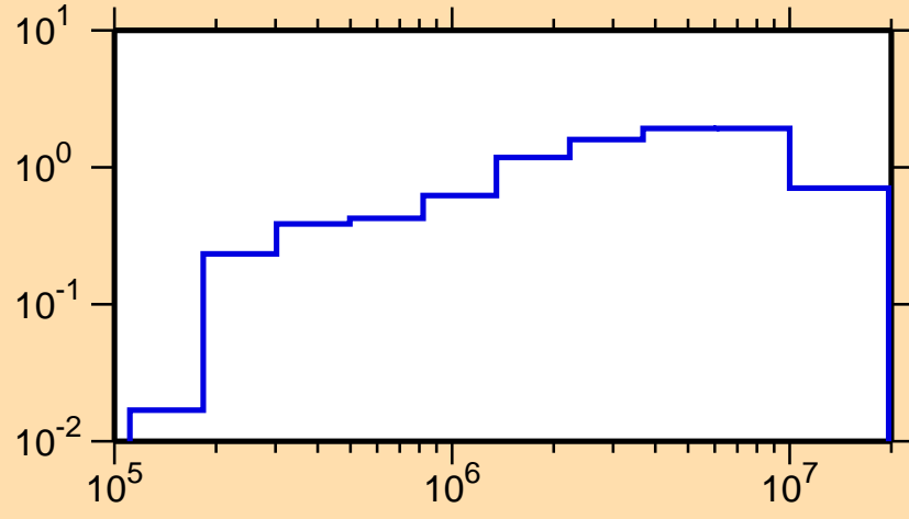
\sigma vs. E for ^{111}\text{Sn}(n,\text{inel.})
