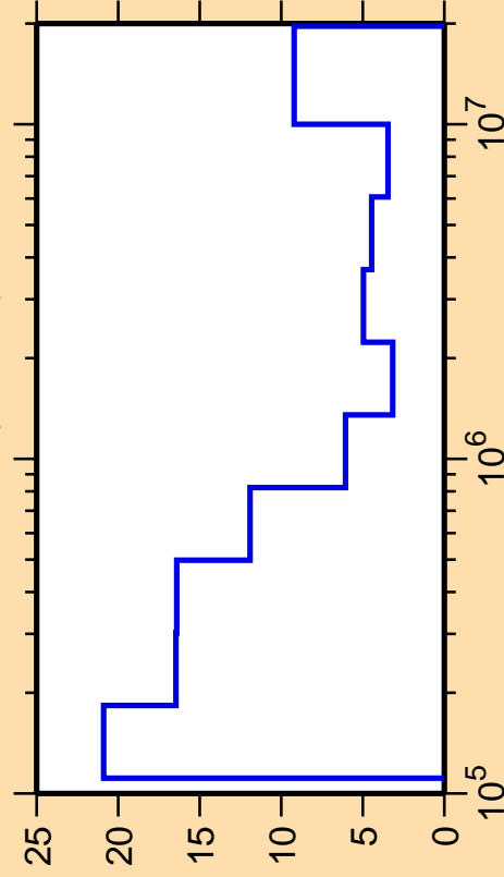
\Delta\sigma/\sigma vs. E for ^{111}\text{Sn}(n,\text{inel.})
