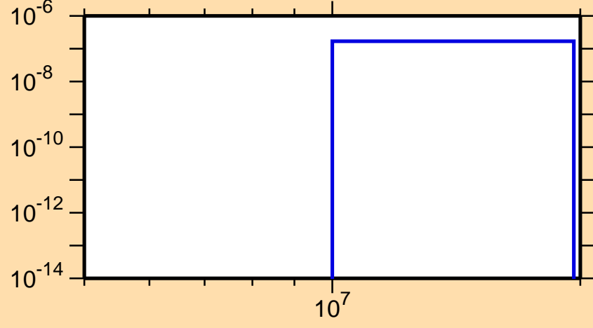
\sigma vs. E for ^{111}\text{Sn}(n,\text{He3})
