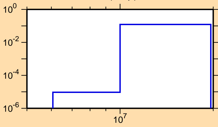
\sigma vs. E for ^{111}\text{Sn}(n,np)
