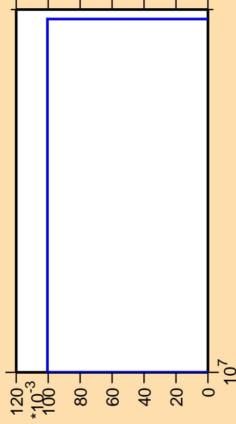
\Delta\sigma/\sigma vs. E for ^{111}\text{Sn} (mt 45)
