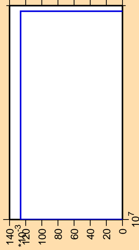
\Delta\sigma/\sigma vs. E for ^{111}\text{Sn}(\text{mt117})
