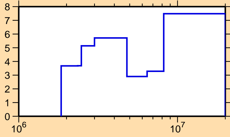
\Delta\sigma/\sigma vs. E for ^{111}\text{Sn}(n,\text{inel.})
