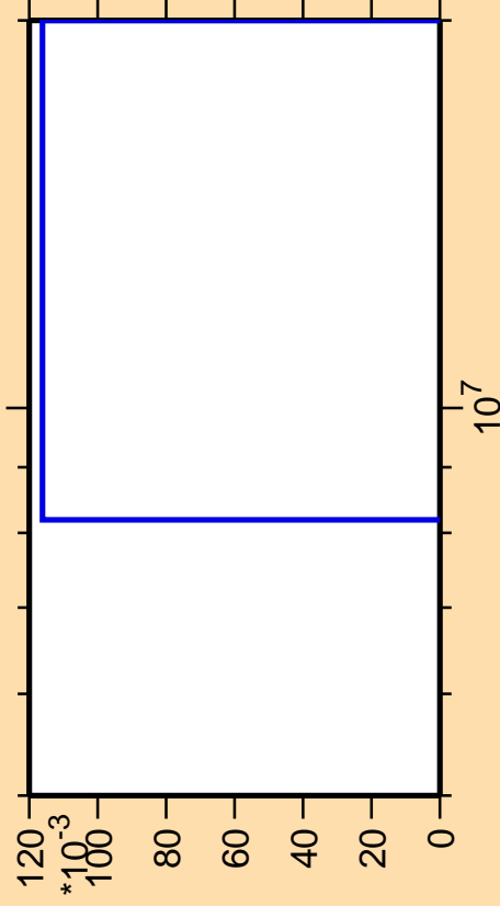
\Delta\sigma/\sigma vs. E for ^{111}\text{Sn}(\text{mt } 45)
