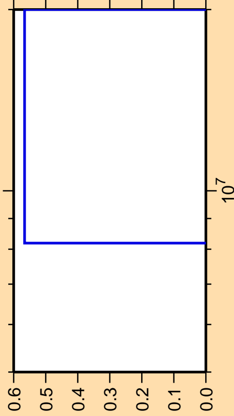
\Delta\sigma/\sigma vs. E for ^{111}\text{Sn}(\text{mt } 34)
