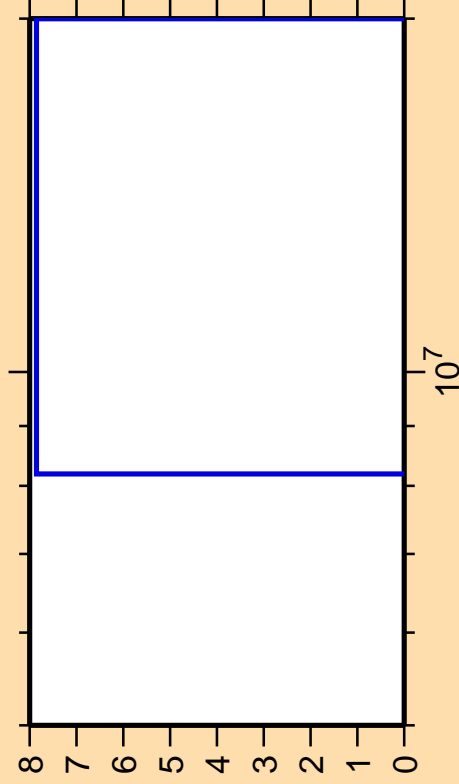
\Delta\sigma/\sigma vs. E for ^{111}\text{Sn}(n,n_1)
