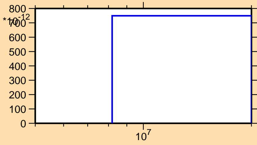
\sigma vs. E for ^{111}\text{Sn}(n,\text{pd})
