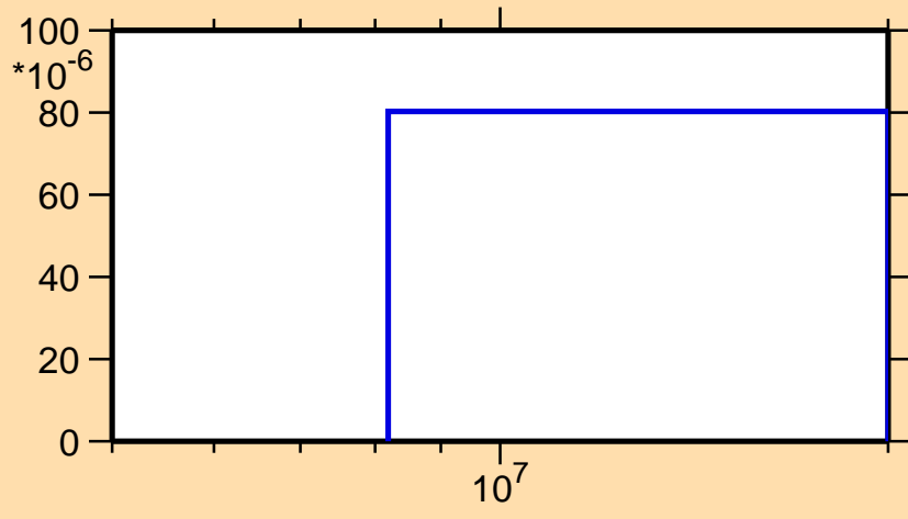
\sigma vs. E for ^{111}\text{Sn}(n,t)
