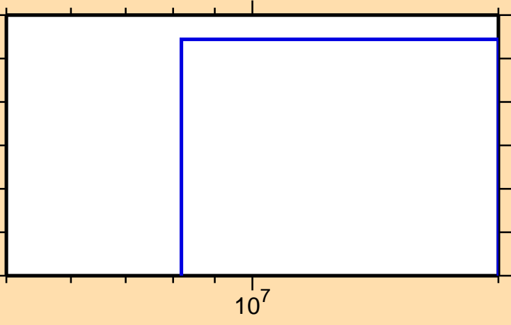
\sigma vs. E for ^{111}\text{Sn}(n,nt)
