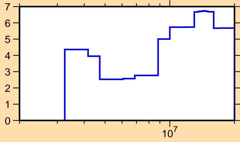
\Delta\sigma/\sigma vs. E for ^{112}\text{Sn}(n,\text{inel.})
