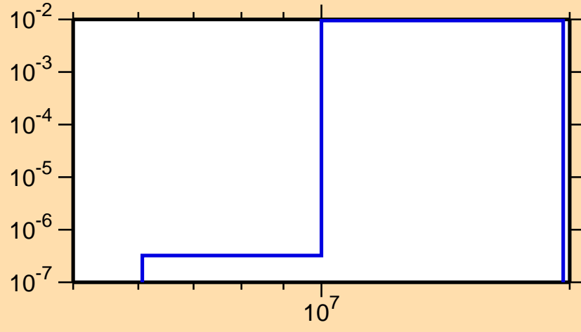
\sigma vs. E for ^{112}\text{Sn}(n,n\alpha)
