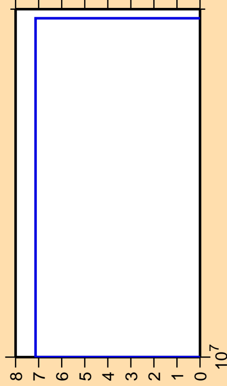
\Delta\sigma/\sigma vs. E for ^{112}\text{Sn}(n,n\text{cont.})
