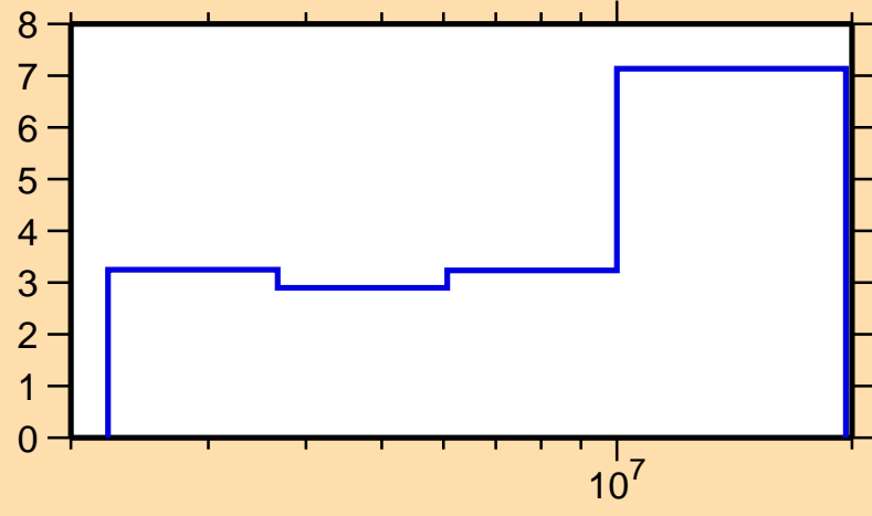
\Delta\sigma/\sigma vs. E for ^{112}\text{Sn}(n,n\text{cont.})
