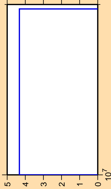
\Delta\sigma/\sigma vs. E for ^{112}\text{Sn}(n,2n)
