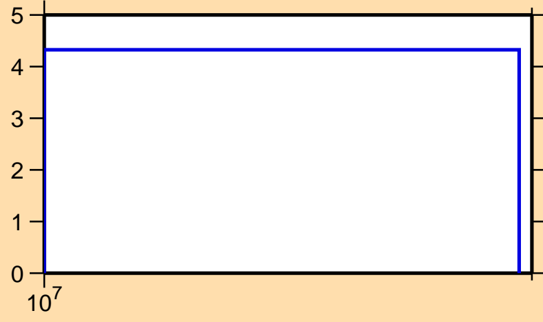
\Delta\sigma/\sigma vs. E for ^{112}\text{Sn}(n,2n)
