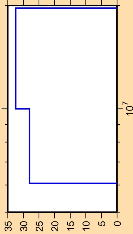
\Delta\sigma/\sigma vs. E for ^{112}\text{Sn}(n,n\alpha)
