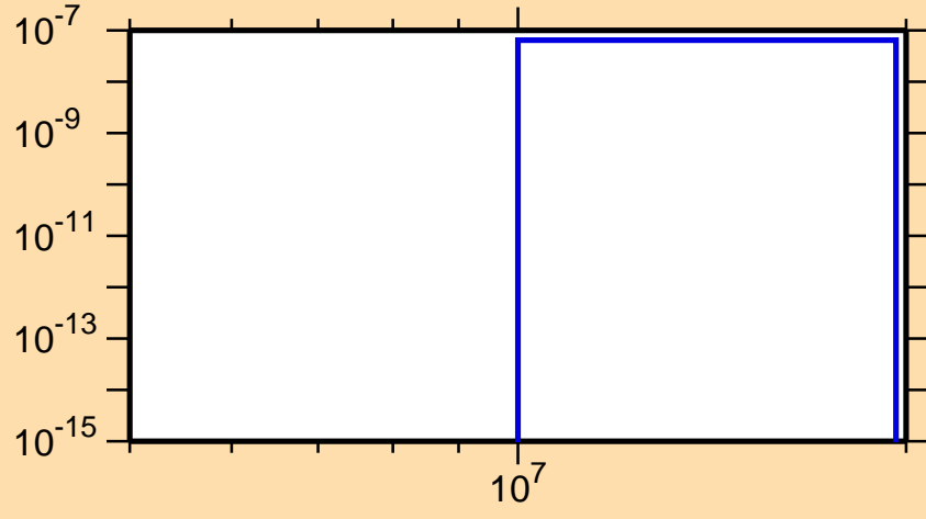
\sigma vs. E for ^{112}\text{Sn}(n,p\alpha)
