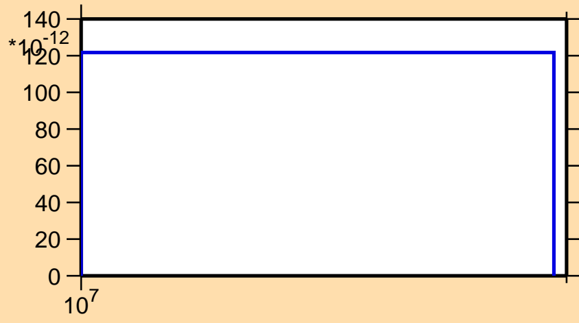
\sigma vs. E for ^{112}\text{Sn}(n,nd)
