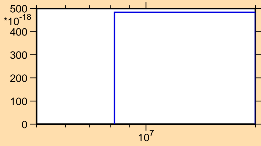
\sigma vs. E for ^{112}\text{Sn}(n,nt)
