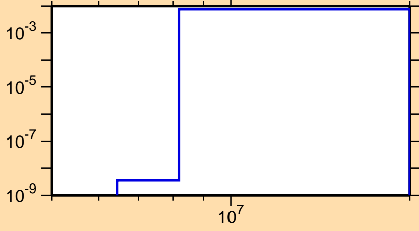
\sigma vs. E for ^{112}\text{Sn}(n,n\alpha)
