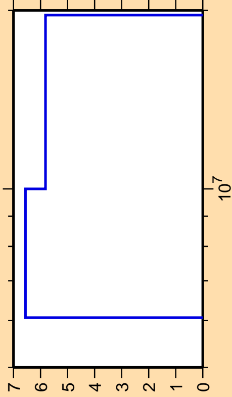
\Delta\sigma/\sigma vs. E for ^{113}\text{Sn}(n,2n)
