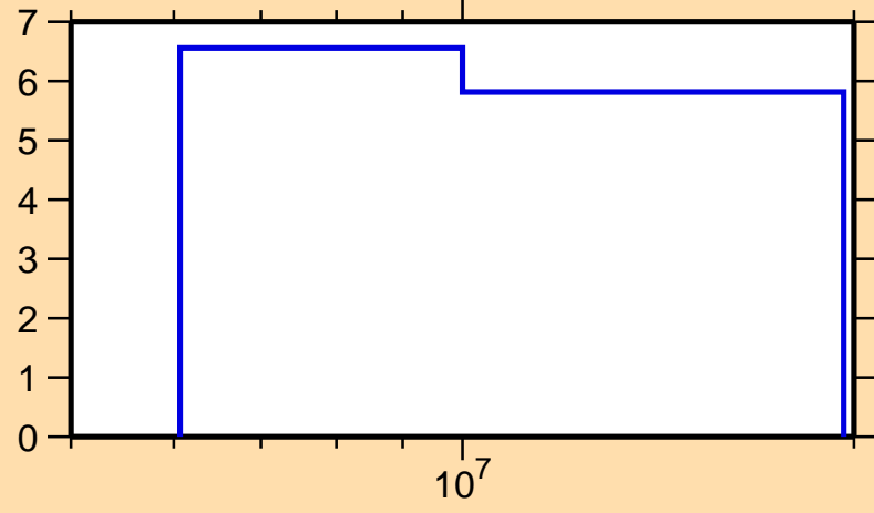
\Delta\sigma/\sigma vs. E for ^{113}\text{Sn}(n,2n)
