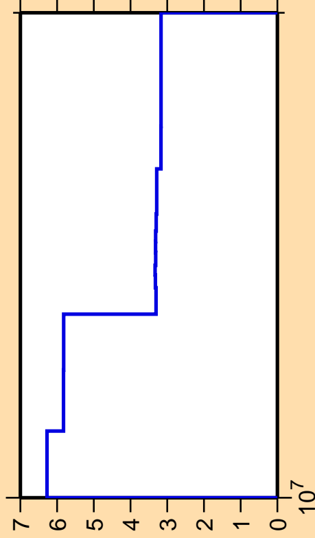
\Delta\sigma/\sigma vs. E for ^{114}\text{Sn}(n,2n)
