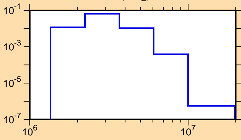
\sigma vs. E for ^{114}\text{Sn}(n,n_2)
