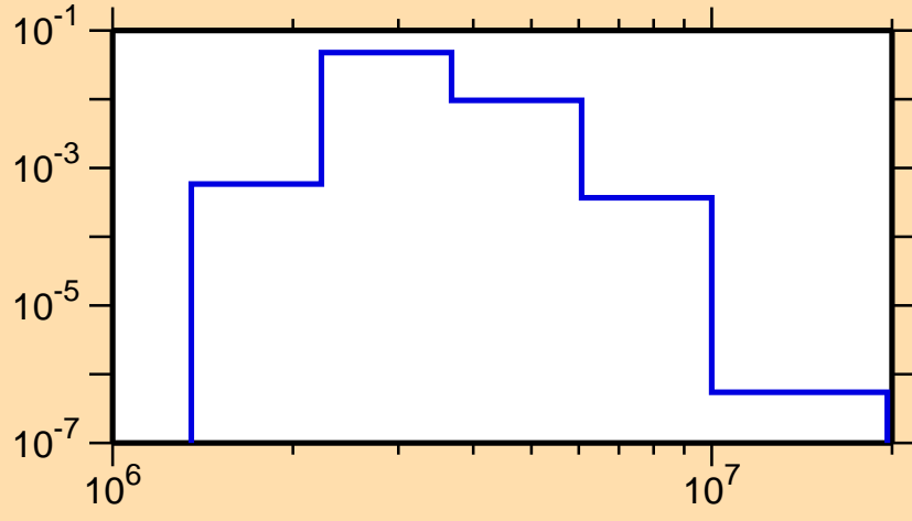
\sigma vs. E for ^{114}\text{Sn}(n,n_3)
