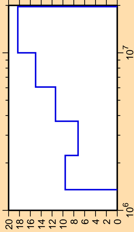
\Delta\sigma/\sigma vs. E for ^{114}\text{Sn}(n,n_3)
