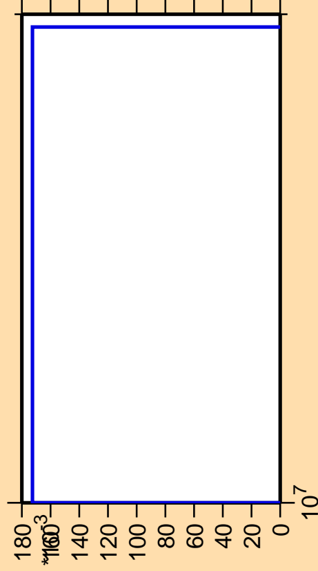
\Delta\sigma/\sigma vs. E for ^{114}\text{Sn}(n,\text{pd})
