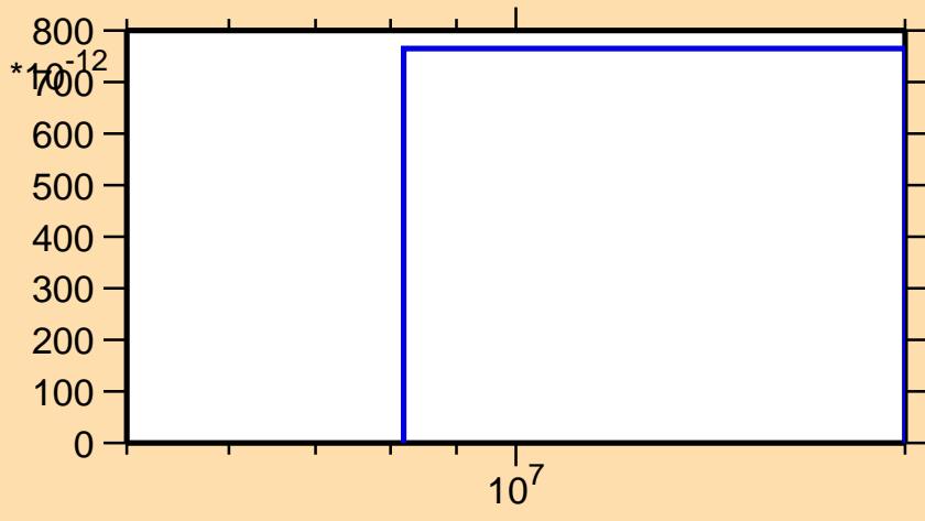
\sigma vs. E for ^{114}\text{Sn}(n,\text{He}3)
