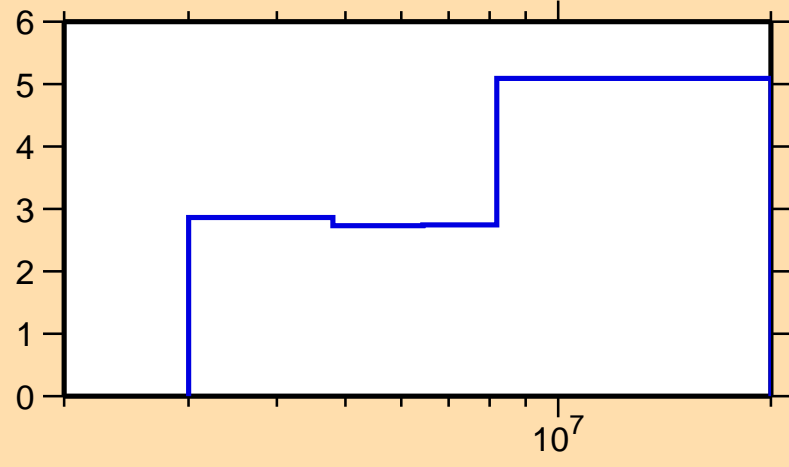
\Delta\sigma/\sigma vs. E for ^{114}\text{Sn}(n,n\text{cont.})
