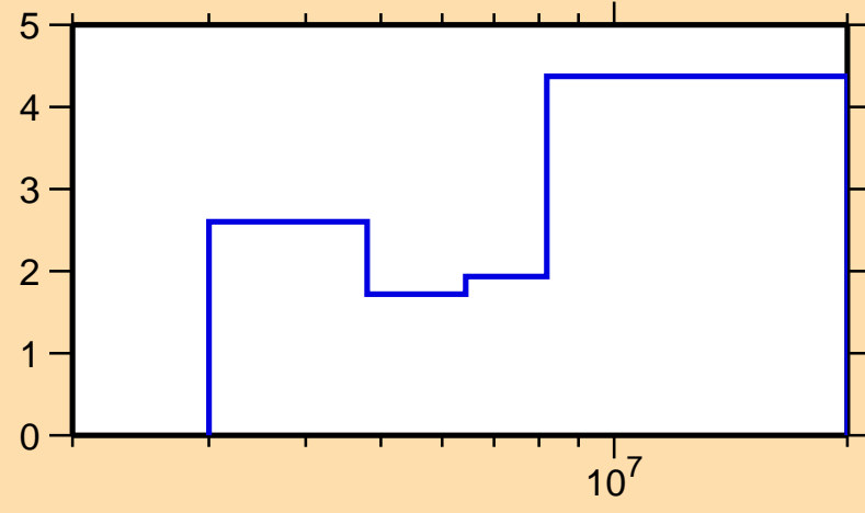
\Delta\sigma/\sigma vs. E for ^{114}\text{Sn}(n,\text{inel.})
