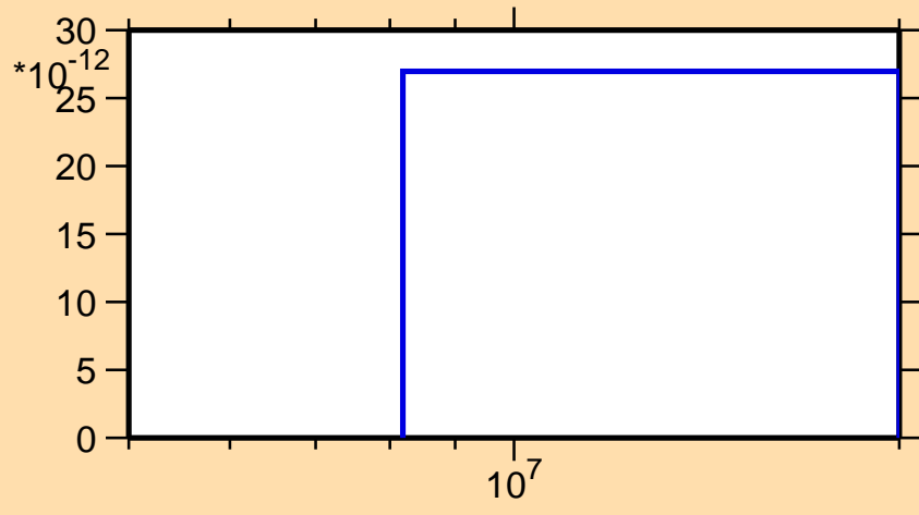
\sigma vs. E for ^{114}\text{Sn}(n,nd)
