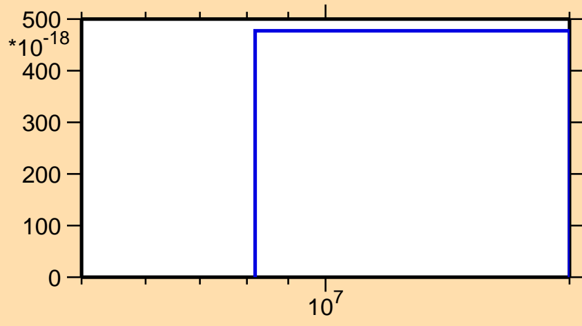
\sigma vs. E for ^{114}\text{Sn}(n,nt)
