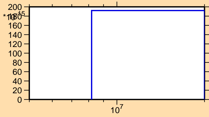
\sigma vs. E for ^{114}\text{Sn}(n,pd)
