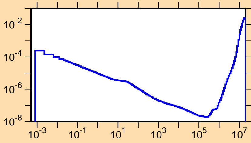
\sigma vs. E for ^{115}\text{Sn}(n,\alpha)
