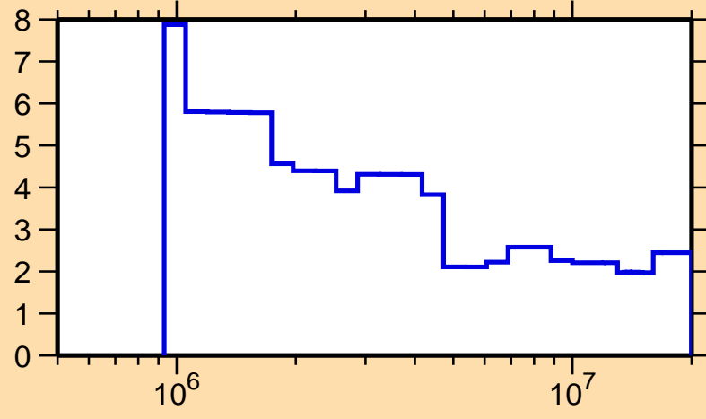
\Delta\sigma/\sigma vs. E for ^{115}\text{Sn}(n,\text{nonel.})
