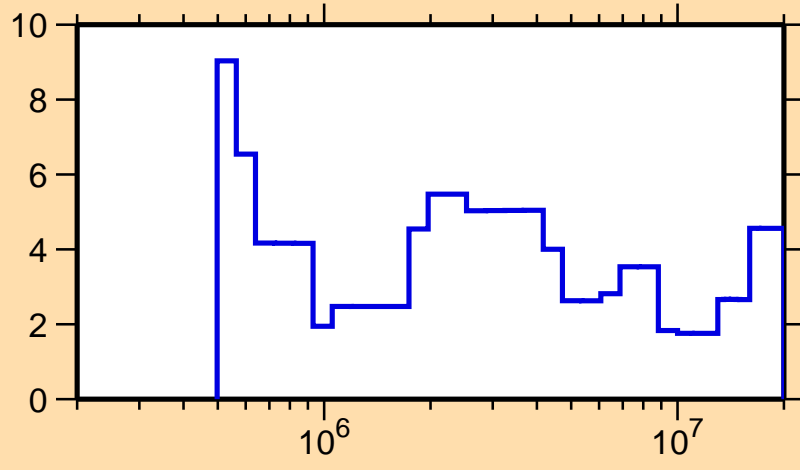
\Delta\sigma/\sigma vs. E for ^{115}\text{Sn}(n,\text{el.})
