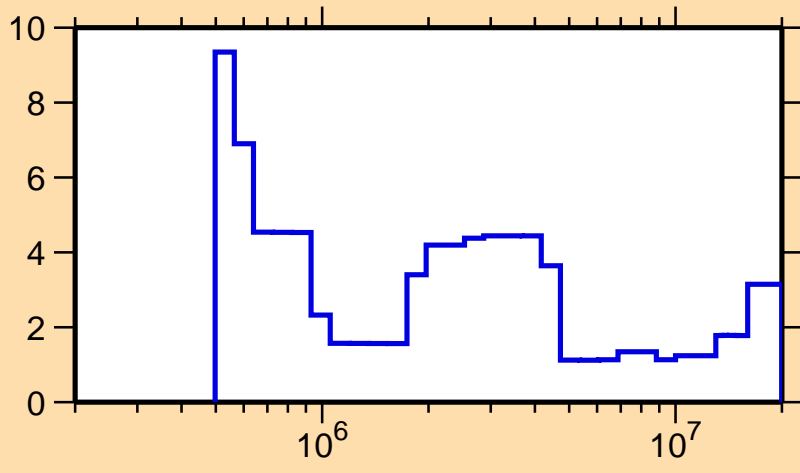
\Delta\sigma/\sigma vs. E for ^{115}\text{Sn}(n,\text{tot.})
