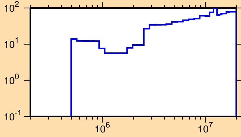
\Delta\sigma/\sigma vs. E for ^{115}\text{Sn}(n,n_1)
