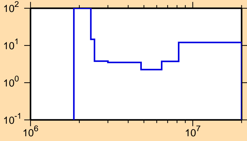
\Delta\sigma/\sigma vs. E for ^{115}\text{Sn}(n,n\text{cont.})
