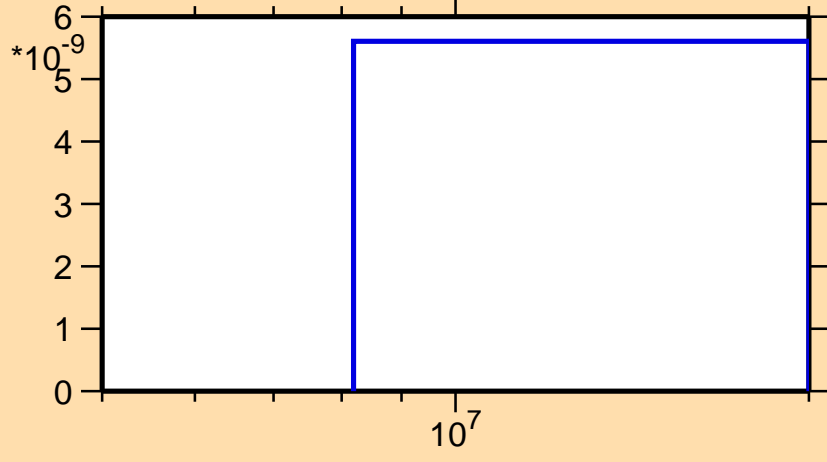
\sigma vs. E for ^{115}\text{Sn}(n,nd)
