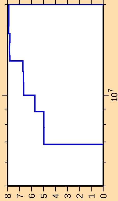
\Delta\sigma/\sigma vs. E for ^{117}\text{Sn}(n,n\text{cont.})
