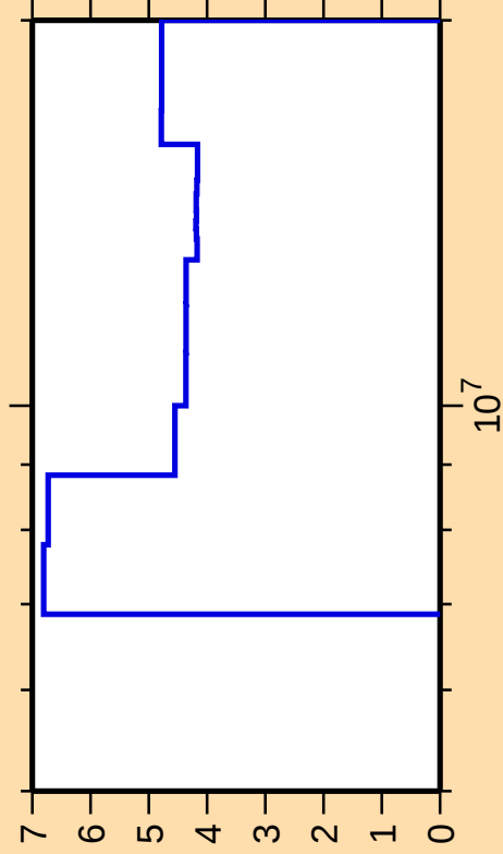
\Delta\sigma/\sigma vs. E for ^{117}\text{Sn}(n,2n)
