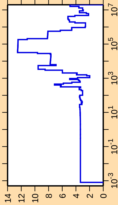
\Delta\sigma/\sigma vs. E for ^{117}\text{Sn}(n,\text{el.})
