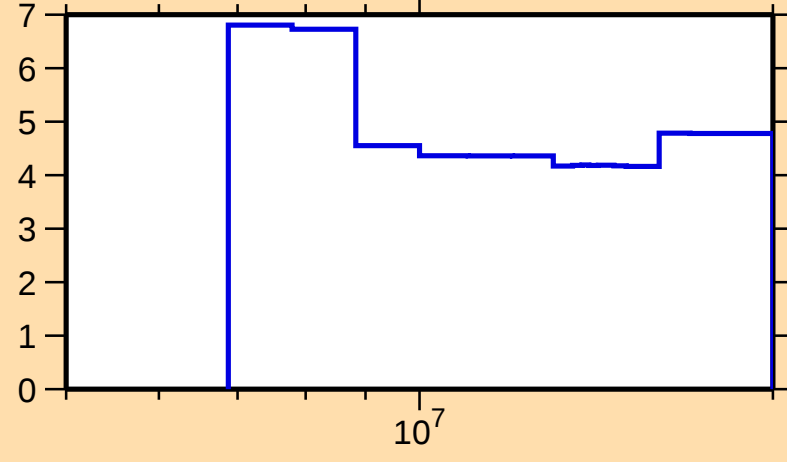
\Delta\sigma/\sigma vs. E for ^{117}\text{Sn}(n,2n)
