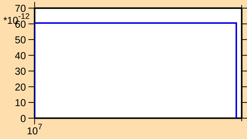
\sigma vs. E for ^{117}\text{Sn}(n,2n\alpha)
