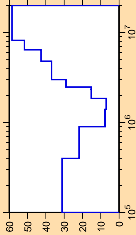
\Delta\sigma/\sigma vs. E for ^{117}\text{Sn}(n,n_4)
