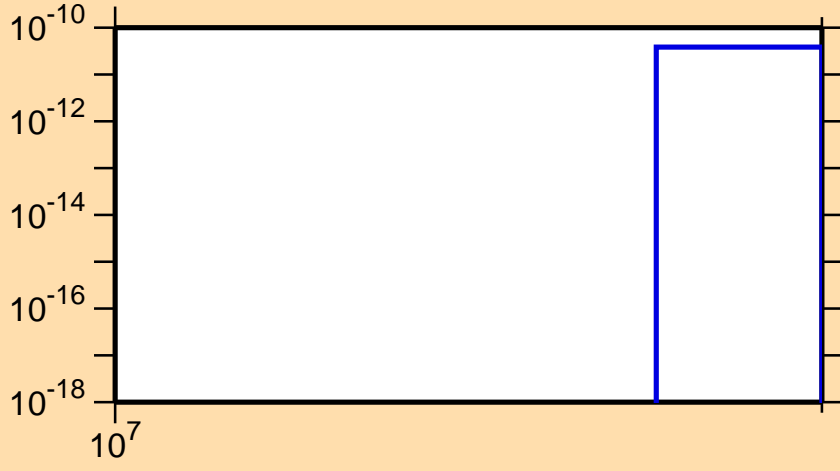
\sigma vs. E for ^{118}\text{Sn}(n,\text{nd})
