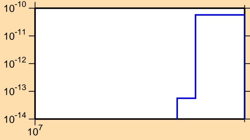
\sigma vs. E for ^{118}\text{Sn}(n,\text{He3})
