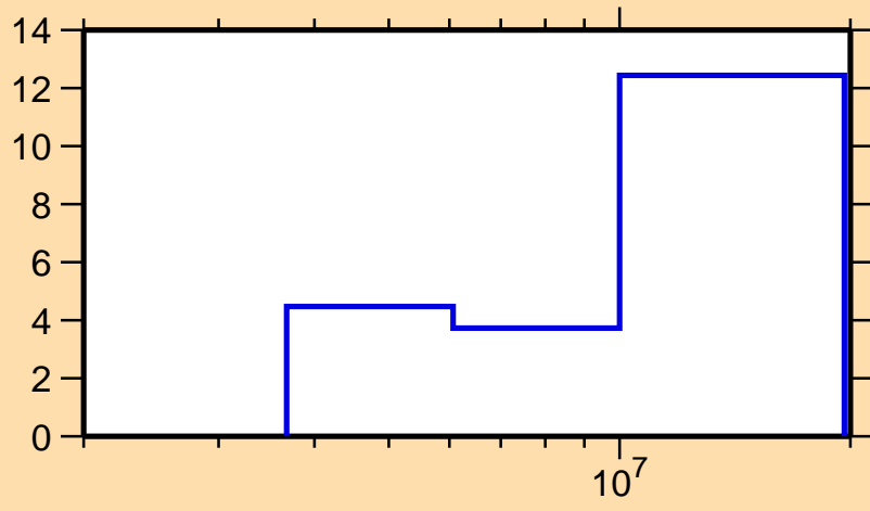
\Delta\sigma/\sigma vs. E for ^{118}\text{Sn}(n,n\text{cont.})
