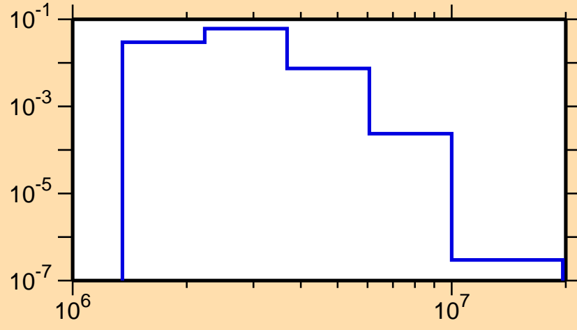
\sigma vs. E for ^{118}\text{Sn}(n,n_2)
