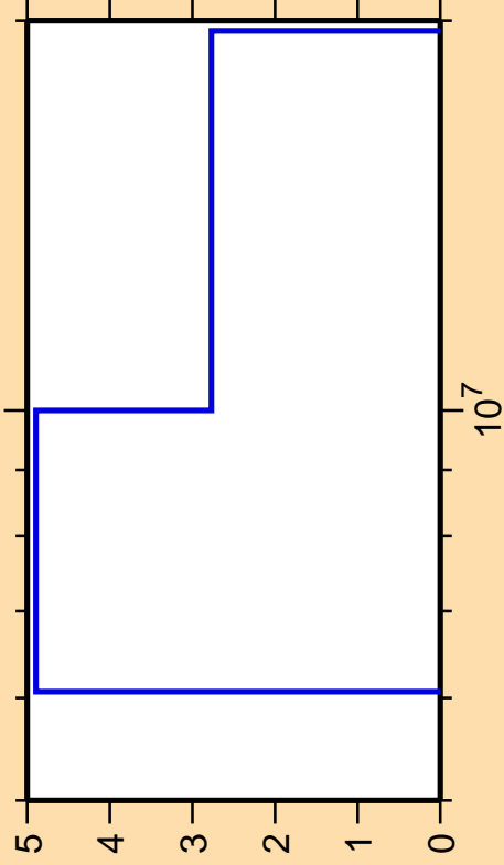
\Delta\sigma/\sigma vs. E for ^{119}\text{Sn}(n,2n)
