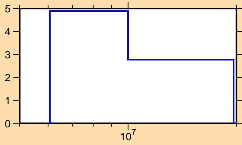
\Delta\sigma/\sigma vs. E for ^{119}\text{Sn}(n,2n)
