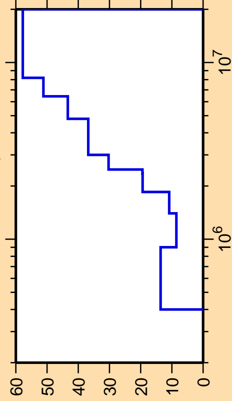
\Delta\sigma/\sigma vs. E for ^{119}\text{Sn}(n,n_3)
