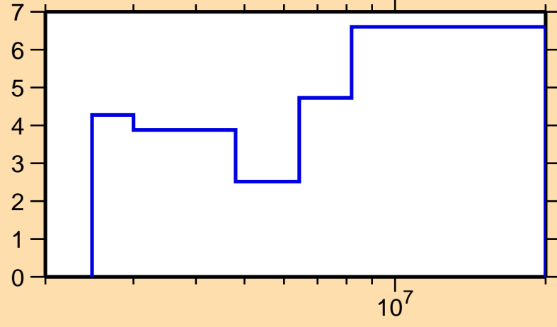
\Delta\sigma/\sigma vs. E for ^{119}\text{Sn}(n,n\text{cont.})
