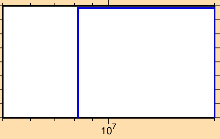
\sigma vs. E for ^{119}\text{Sn}(n,2n\alpha)
