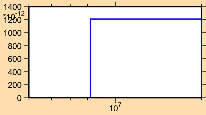
\sigma vs. E for ^{119}\text{Sn}(n,nd)
