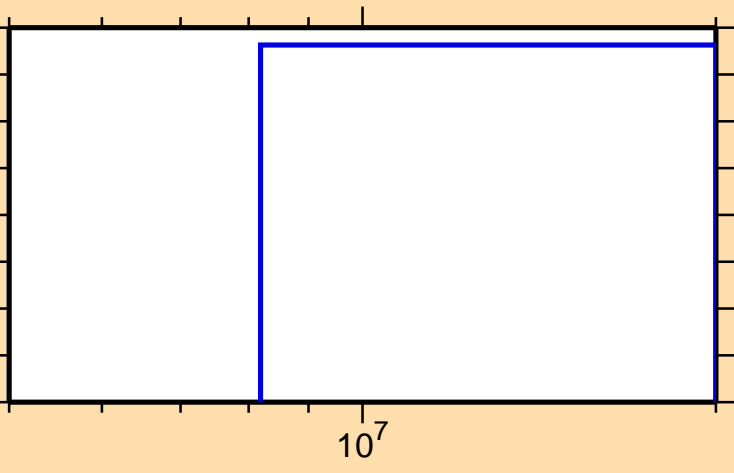
\sigma vs. E for ^{119}\text{Sn}(n,2np)
