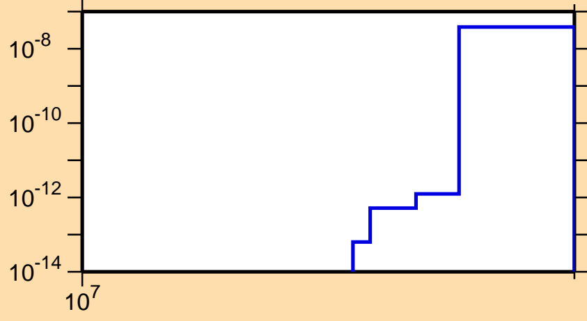
\sigma vs. E for ^{121}\text{Sn}(n,nd)
