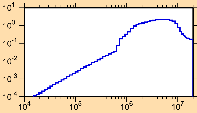
\sigma vs. E for ^{121}\text{Sn}(n,\text{inel.})
