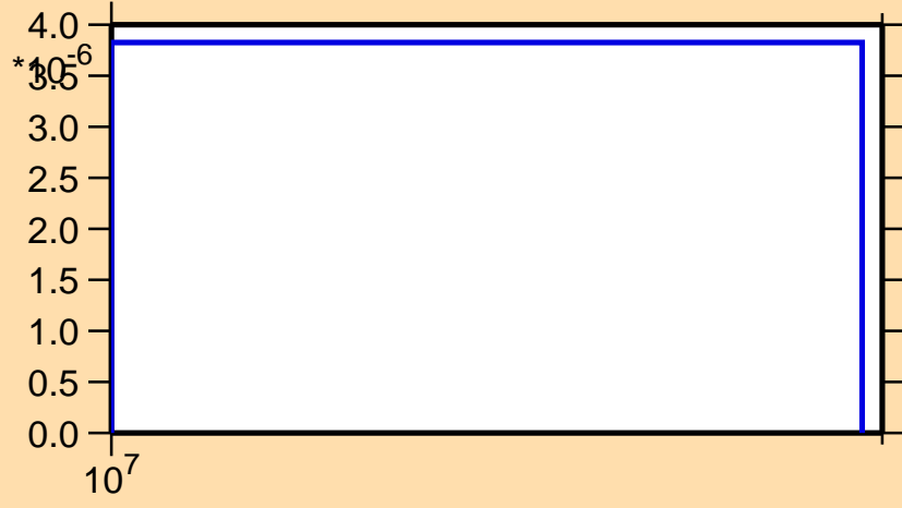
\sigma vs. E for ^{121}\text{Sn}(n,t)
