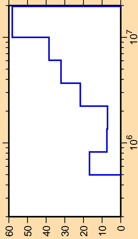
\Delta\sigma/\sigma vs. E for ^{121}\text{Sn}(n,n_3)
