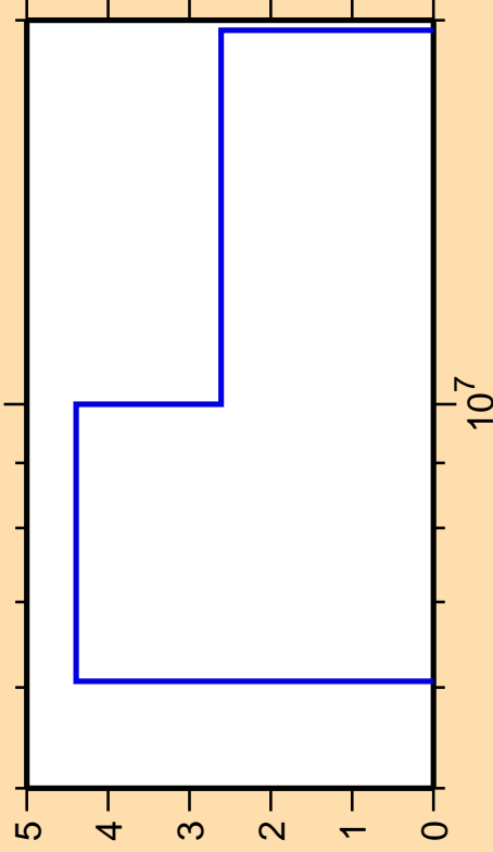
\Delta\sigma/\sigma vs. E for ^{121}\text{Sn}(n,2n)
