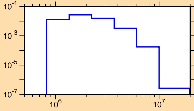
\sigma vs. E for ^{121}\text{Sn}(n,n_4)
