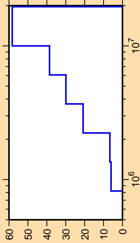
\Delta\sigma/\sigma vs. E for ^{121}\text{Sn}(n,n_4)
